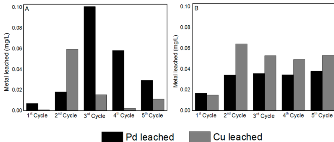
Figure S4. Pd and Cu leached during stability experiments performed with: (A) 5% Pd-2.5% Cu/CNT(BM 2h) and (B) 2.5% Pd-2.5% Cu/CNT(BM 2h).
