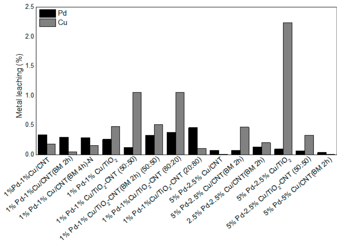
Figure S3. Pd and Cu leached during NO 3 - catalytic reduction experiments performed for all the synthesized catalysts.
