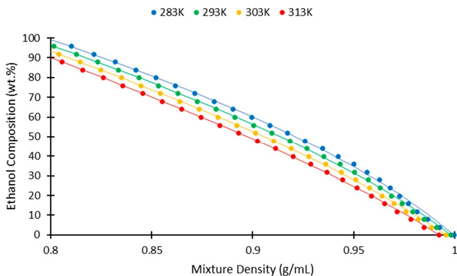
Figure S1: Global comparison of the Redlich-Kister model fit to literature density data between 0-100 wt.% ethanol. Data points represent published data and trend lines represent model fit.
