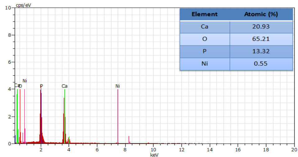
Figure 5. EDAX spectrum of Ni 2+ -doped HApNPs calcined at 500 °C.
