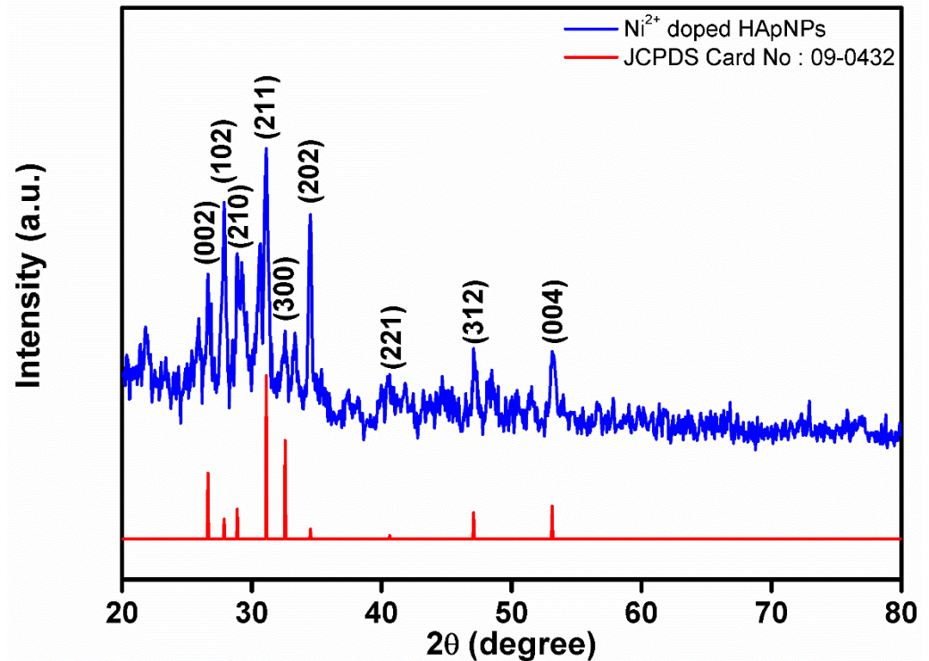
Figure 1. XRD analysis of Ni 2+ -doped HApNPs calcined at 500 °C.
