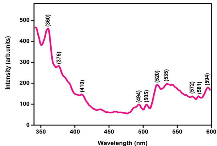
Figure 6. PL emission spectrum of Ni 2+ -doped HApNPs calcined at 500 °C.
