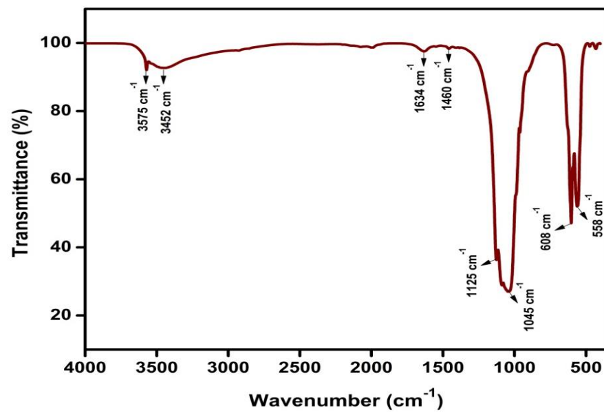
Figure 2. FTIR spectrum of Ni 2+ -doped HApNPs calcined at 500 °C.
