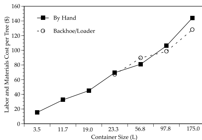
Figure 2. Labor and materials cost [US$] per tree for transplant by hand or machinery of various container size trees in 2013 (excluding wholesale cost of tree) as determined from RSMMeans [23].
