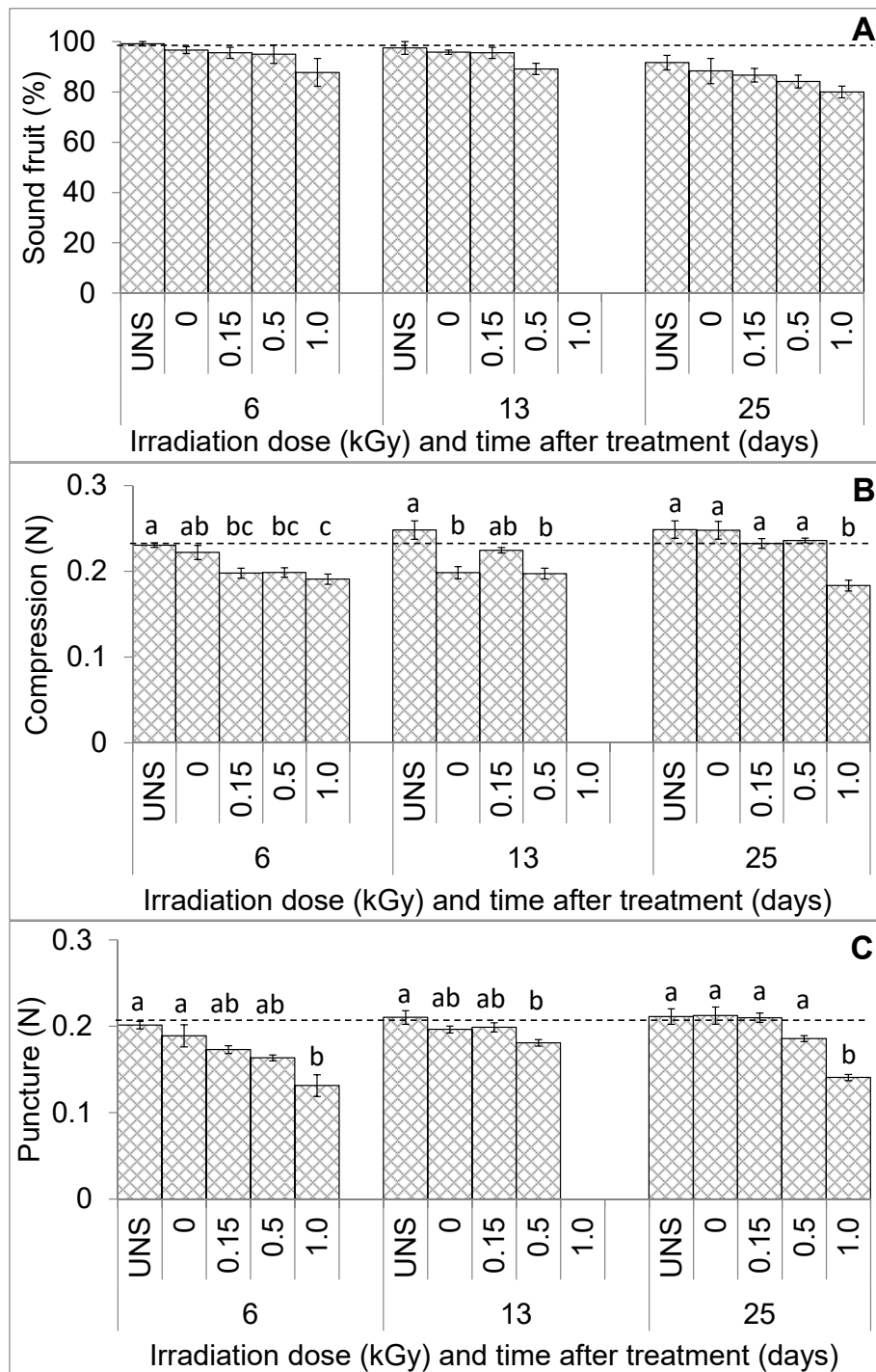
Figure 2. Effect of Electronic Cold-Pasteurization™ on percent sound fruit (A), compression (B), and puncture (C) for ‘Farthing’ blueberries in trial 2. Treatments included an unshipped control (UNS; not shipped to the irradiation facility) and four levels of irradiation; no irradiation control (0), 0.15, 0.5, and 1.0 kGy. Evaluations were conducted 6, 13, and 25 days after irradiation treatment. Fruit were stored at 2 to 4 °C under high relative humidity until assessments were performed. An initial fruit quality assessment was performed after harvest shown as a horizontal dashed line. Due to low number of fruit, measurements were not performed for fruit treated at 1 kGy at 13 days after treatment. Means within the same storage times after treatment followed by the same letter are not significantly different from each other based on one-way analysis of variance ( \alpha = 0.05 ).
