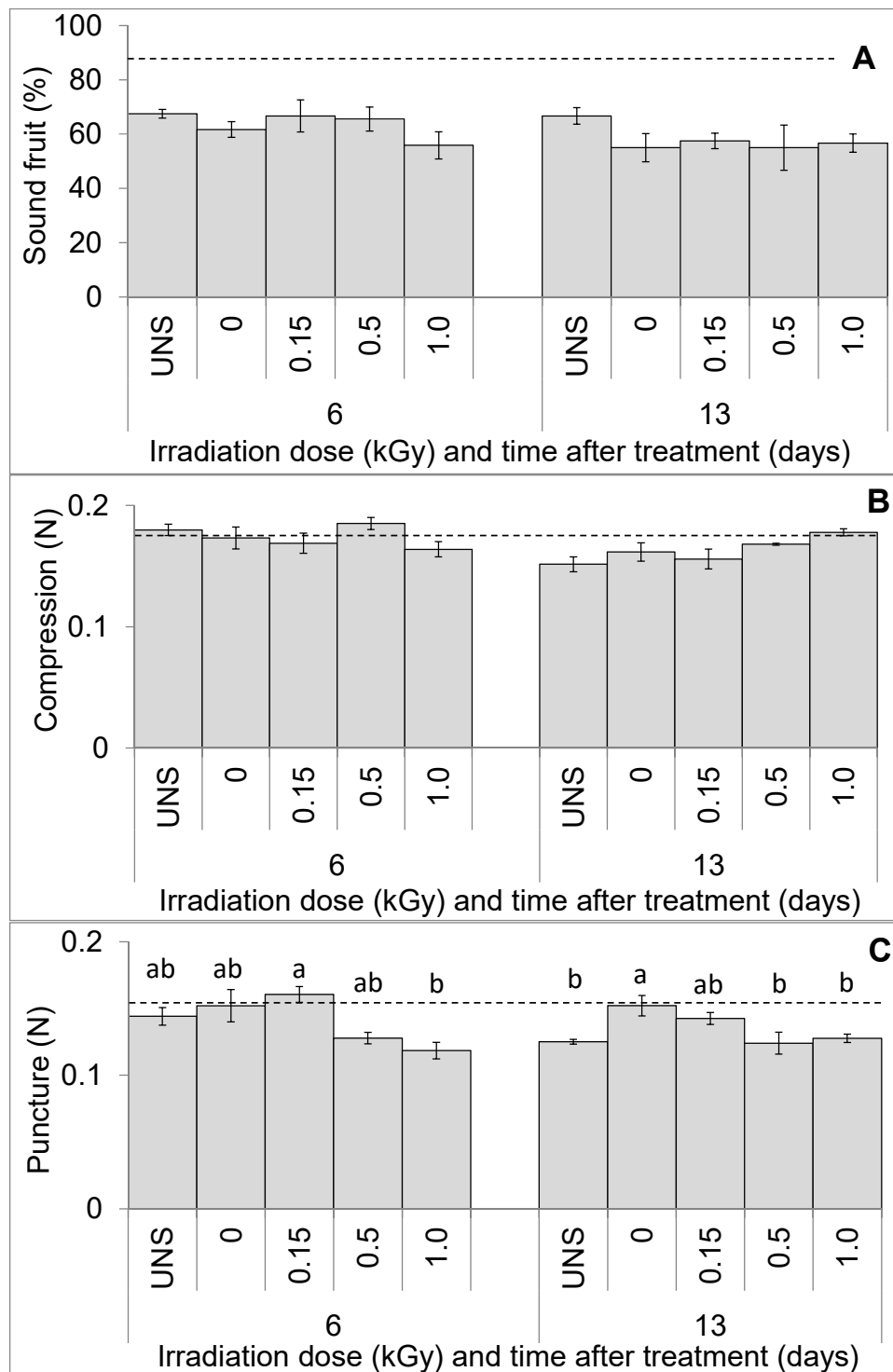
Figure 3. Effect of Electronic Cold-Pasteurization TM on percent sound fruit (A), compression (B), and puncture (C) for ‘Rebel’ blueberries in trial 2. Treatments included an unshipped control (UNS; not shipped to the irradiation facility) and four levels of irradiation; no irradiation control (0), 0.15, 0.5, and 1.0 kGy. Evaluations were conducted 6 and 13 days after irradiation treatment. Fruit were stored at 2 to 4 °C under high relative humidity until assessments were performed. An initial fruit quality assessment was performed after harvest shown as a horizontal dashed line. Means within the same storage times after treatment followed by the same letter are not significantly different from each other based on one-way analysis of variance ( \alpha = 0.05 ).
