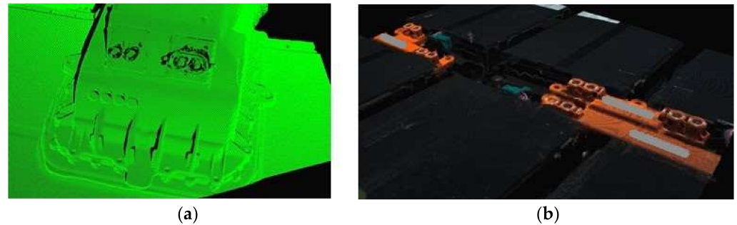
Figure 8. Point cloud of the switch box (a), modules and busbars (b) that were captured with Zivid Two.
