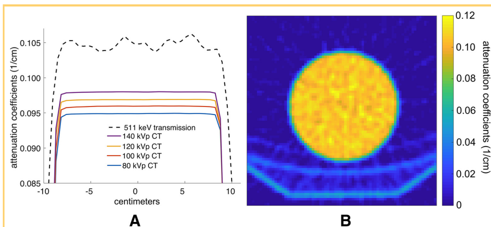
Figure 5. Profiles showing CT-based attenuation estimates in the solid epoxy phantom as well as 511-keV transmission measurement (dashed line) (A). The attenuation image produced using 511-keV photons (B).
