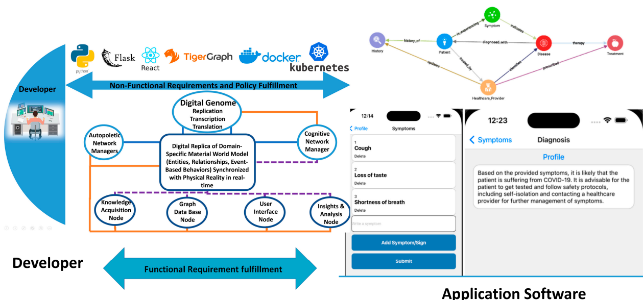
Figure 3. Architecture of medical knowledge-based digital assistant.
