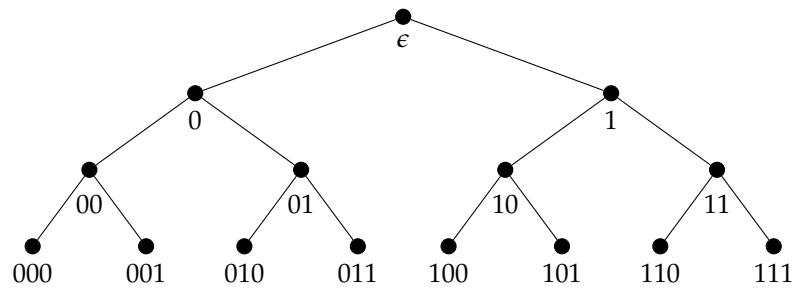
Figure 2. The perfect binary tree t_3^* with nodes labeled by binary strings
