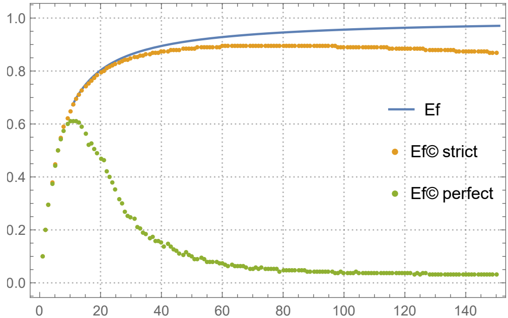
Figure 5. Dependencies of Ef and Ef ⊙ on the number of positions.
