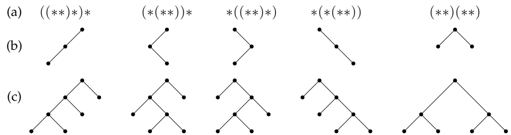
Figure 1. Images of the free magma: (a) bracketing, (b) non-strict binary tree, (c) strict binary tree.
