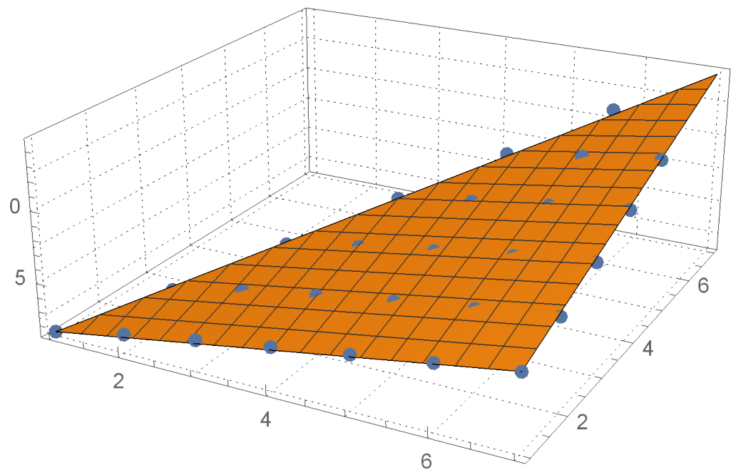
Figure 6. Average heights of generated trees and their linear approximation for m = 8 .
