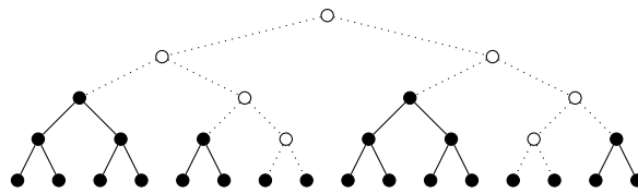
Figure 3. Example of a perfect binary forest.
