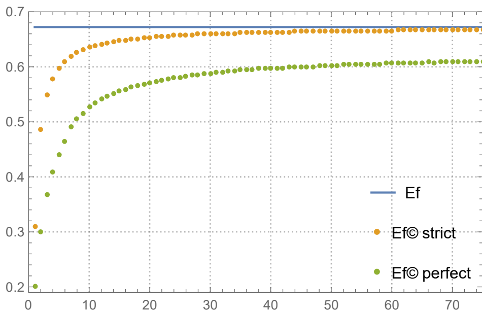
Figure 4. Dependencies of Ef^{\circledast} on the number of blocks for n_{st} = n_{pr} = n_{pos} = 5 .
