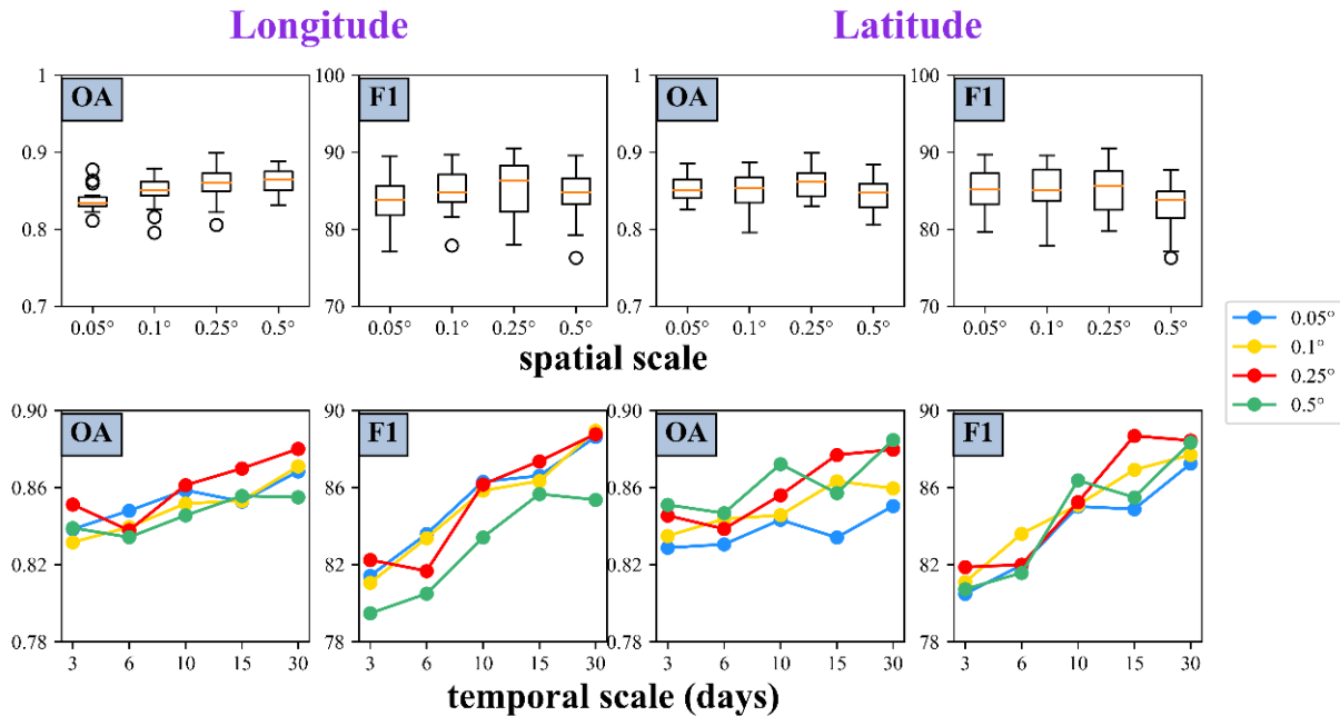
Figure 8. Dispersion and trend of model performance at different temporal and spatial scales (longitude and latitude).
