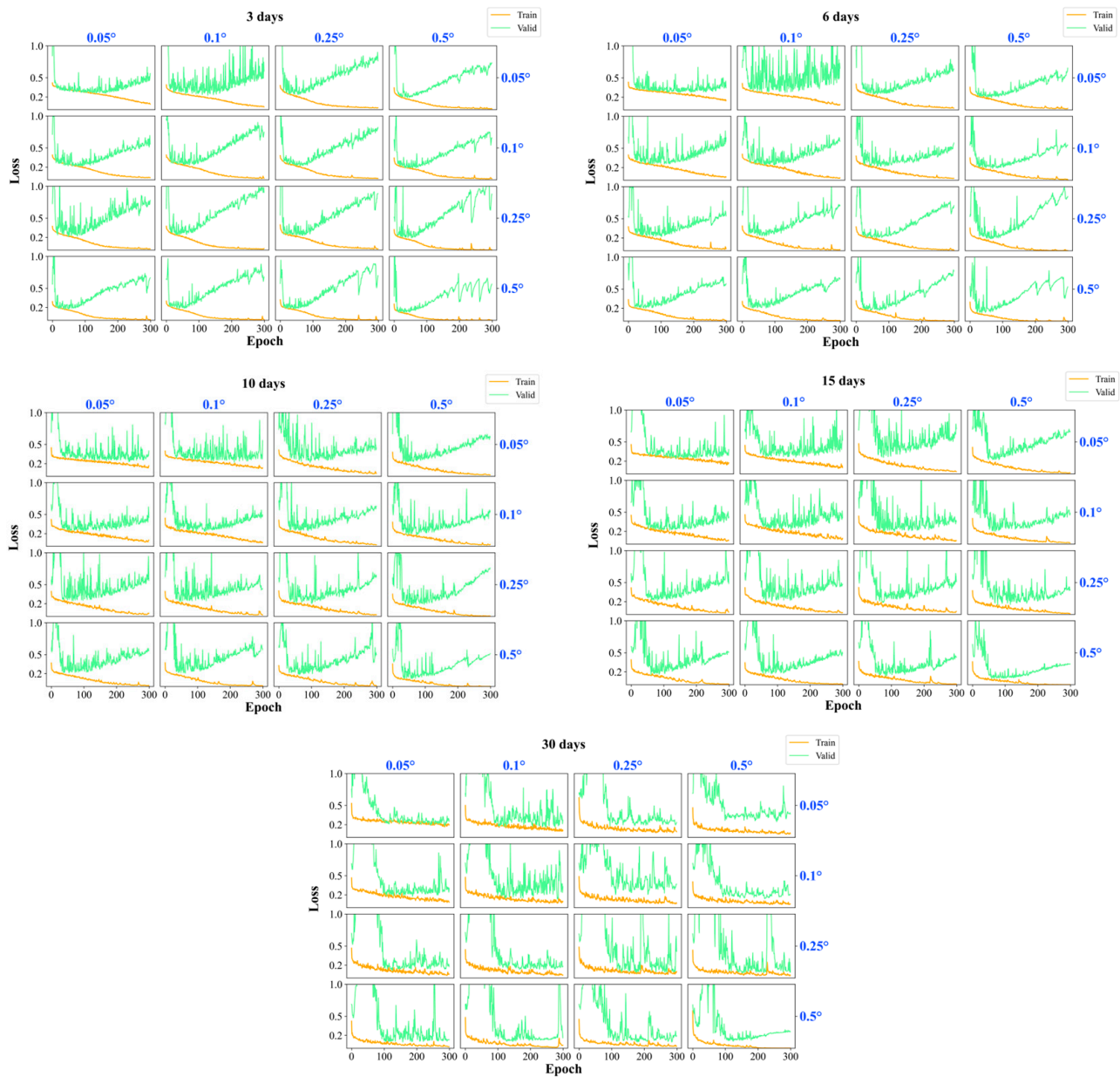
Figure 4. Loss curves of the training and validation sets of the fishing ground prediction model in different temporal and spatial scales. Train and Valid in the figure represent the training and validation sets, respectively.
