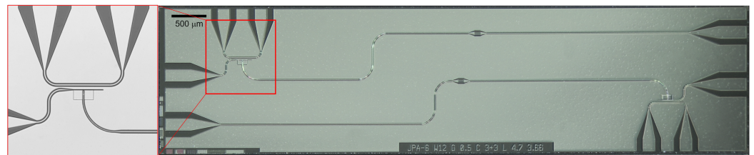
Figure 3. Microscope picture of the chip comprising two JPA devices. Each JPA device consists of an aluminum resonator terminated with a dc-SQUID, a pump transmission line and a dc-flux line.
