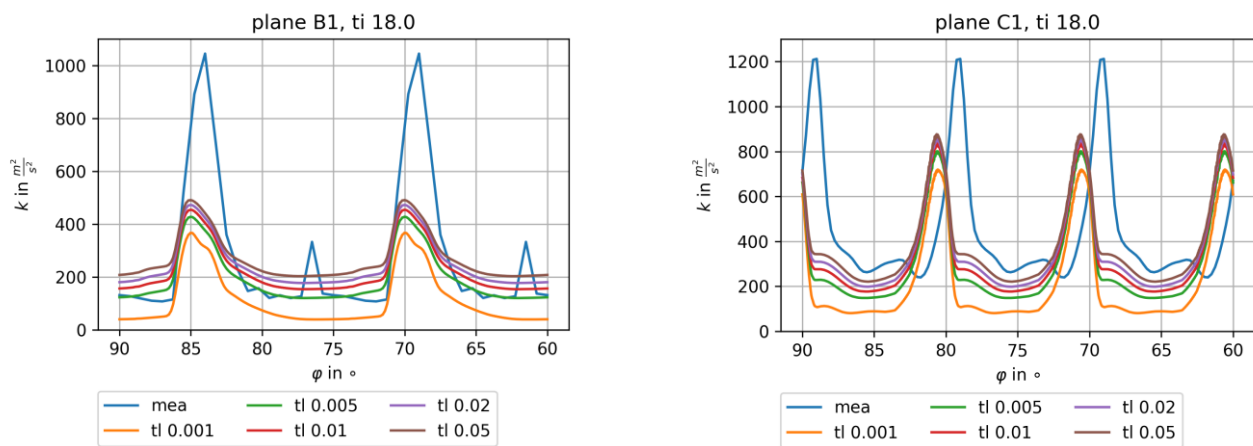
Figure 5. Comparison of turbulence kinetic energy in planes B1 (left) and C1 (right) for an inlet turbulence intensity of 18% and varying turbulence length scale (1–50 mm) (mea . . . measured) (Q3D simulation at mid-section).
