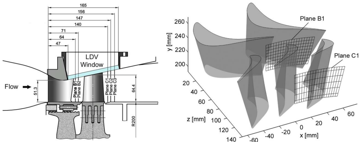
Figure 1. Meridional view of flow channel (left) and blade contours with measurement planes (right).
