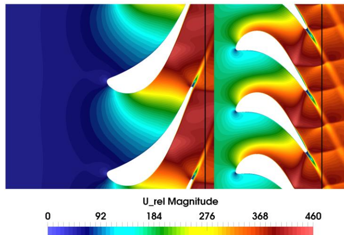
Figure 3. Absolute (stator) and relative velocity (rotor) at mid-span (steady solution).
