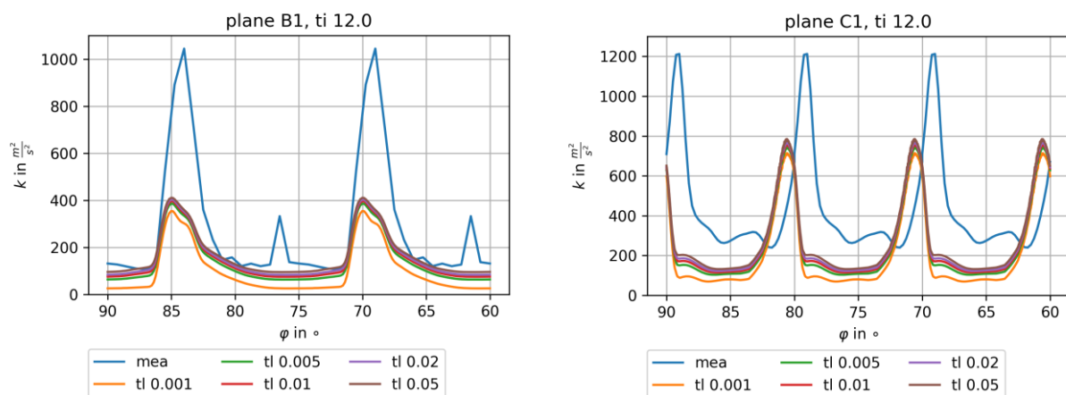
Figure 4. Comparison of turbulence kinetic energy in planes B1 (left) and C1 (right) for an inlet turbulence intensity of 12% and varying turbulence length scale (1–50 mm) (mea . . . measured) (Q3D simulation at mid-section).
