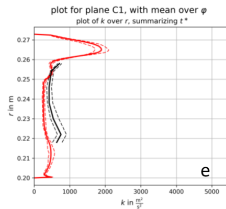
Figure 12. (a–d) Circumferentially averaged turbulence kinetic energy and minimum and maximum values in plane C1 at different time instants; (e) Time average of all mean distributions with variations (black: experiments; red: computations).
