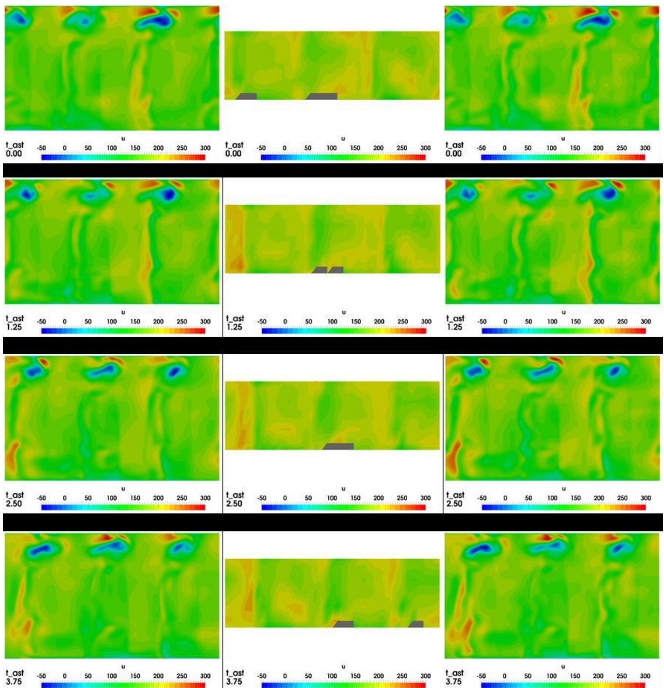
Figure 10. Instantaneous measured (middle) and computed (left: 18%/5 mm inlet turbulence, right: 12%, 1 mm inlet turbulence) velocity in plane C1 after the rotor (view in upstream direction).
