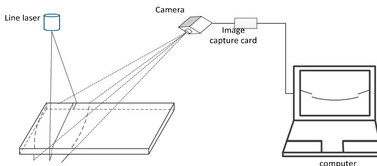
Figure 2. Image acquisition system of the fisheye.
