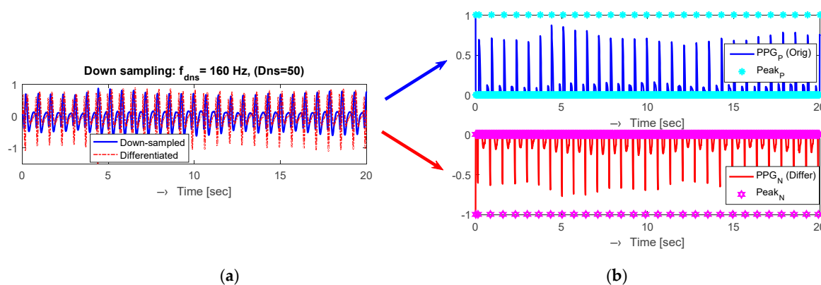
Figure 1. An example of PPG signal processing in a 20-s ROI: down-sampled signal (originally recorded at f_s = 8 kHz together with its first derivative (a), positive/negative peak positions of the down-sampled/differentiated PPG signal (b).
