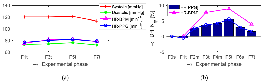
Figure 5. Partial comparison of values measured by the BPM device and determined from the PPG signal: BP and HR values in four measuring phases (a); relative differences in [%] between N_{tp}/HR values determined from the PPG signal/by the BPM device in all eight experimental phases relative to the F0s/F1t as a baseline (b), for the male tested person, experiment no. 2.
