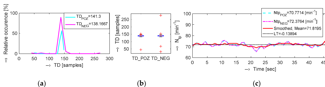
Figure 2. Second phase of PPG signal processing: (a) histograms of time distances between localized peaks for both signal polarities; (b) box plot of basic statistical analysis of TD values; (c) curves from both polarities of the signal, their smoothing, and the linear trend for the whole recorded PPG signal.
