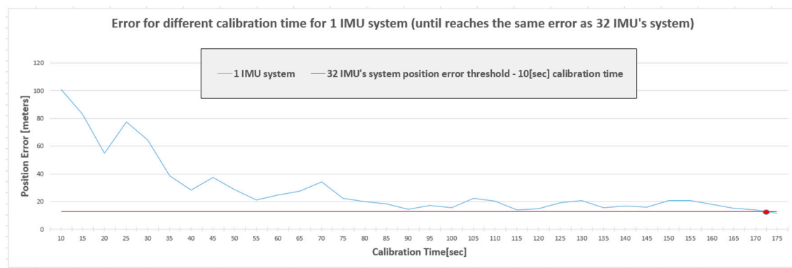
Figure 2. Position error of 1 IMU system dependent on the calibration time of this system (blue curve). Table 32 components MIMU system with 10 s of calibration. The time of the point where the blue and red curves meet, represents the calibration time needed from 1 IMU system to receive the same error as the 32 components MIMU system.
