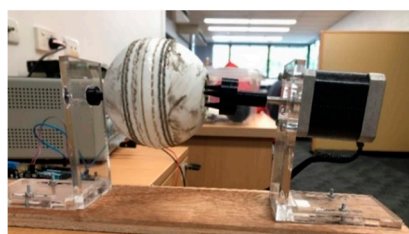
Figure 3. Microcontroller calibration setup.
