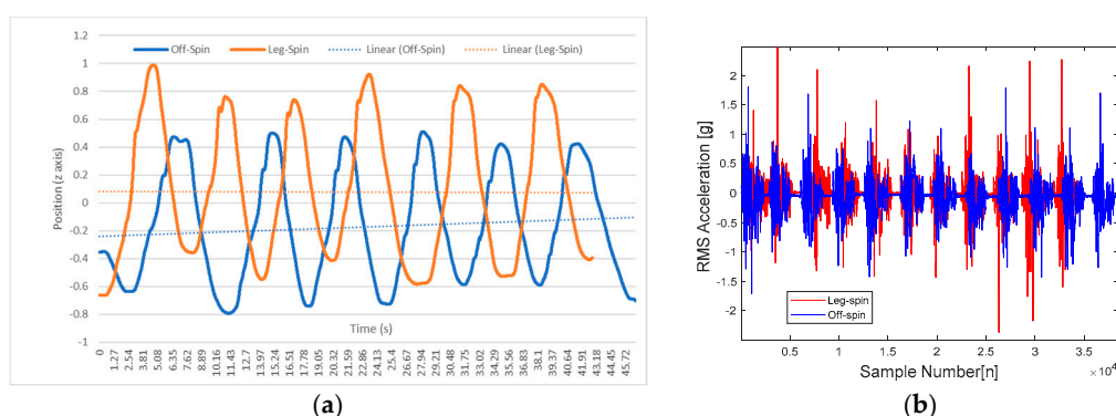
Figure 7. Linear classification model for off-spin and leg-spin bowlers: (a) motion capture; (b) root mean square (RMS) acceleration of the bowler’s lumbar (T3) using IMU sensors sampled at 250 Hz.
