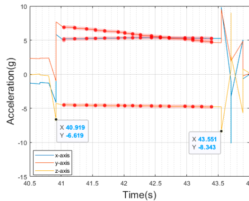
Figure 5. Flight time measurements of a spinning ball.
