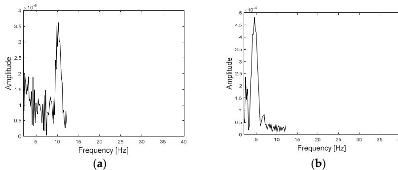
Figure 6. (a) Frequency domain for leg-spin balls; (b) frequency domain for off-spin balls.
