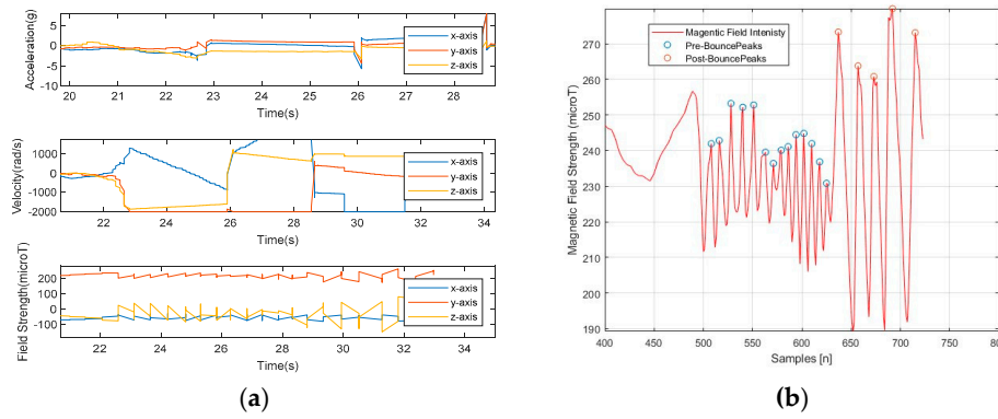
Figure 4. (a) IMU sensor readings of a spinning ball (acceleration—top, gyroscope—middle and magnetometer—bottom); (b) pre-bounce and post-bounce peaks of a spinning ball for the magnetometer.
