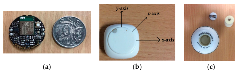
Figure 1. (a) MetaWear CPRO (mbientlab.com); (b) axes orientation on the MetaWear CPRO sensor placed inside a plastic case; (c) insertion of the sensor into the side of an indoor cricket ball.
