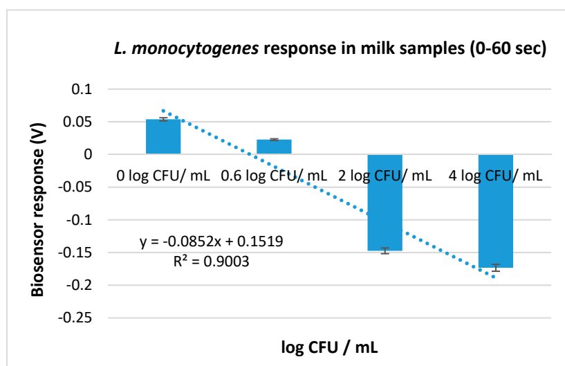
Figure 5. L. monocytogenes response in milk samples with four different initial concentrations (0, 0.6, 2, and 4 log CFU mL -1 ) after incubation with the primary enrichment broth. The error bars represent the standard errors of the mean value of all replications. The columns are marked with different letters, indicating that response was significantly ( p < 0.05 ) different from the respective of the control samples (samples incubated with the primary enrichment without L. monocytogenes (0 log CFU mL -1 )) for each experimental assay.
