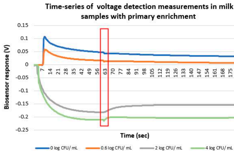
Figure 4. Time series of the 360 voltage detection measurements obtained from four different electrodes testing milk samples with four different L. monocytogenes concentrations (0, 0.6, 2, and 4 log CFU mL -1 ) after incubation with the primary enrichment broth. Samples were added on each electrode and measurements were recorded for 60 s. The biosensors were then added (red box) and the measurements recorded describe the reaction between the sample and the biosensor (60–180 s/120–360 measurements).
