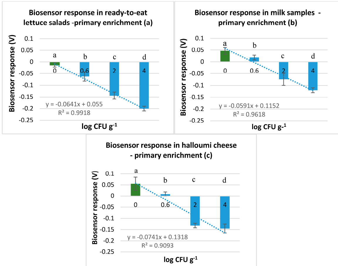
Figure 2. Biosensor response in (a) ready-to-eat lettuce salad samples, (b) milk samples and (c) halloumi cheese samples without L. monocytogenes (green color) and with L. monocytogenes (blue color) at 0.6, 2 and 4 log CFU g -1 (initial inoculation level) after incubation with primary enrichment broth (Half Fraser). The error bars represent the standard errors of the mean value of all replications. The columns marked with different letters indicate that response was significantly ( p < 0.05 ) different from the respective of the control samples (samples without L. monocytogenes incubated with the primary enrichment) for each experimental assay.
