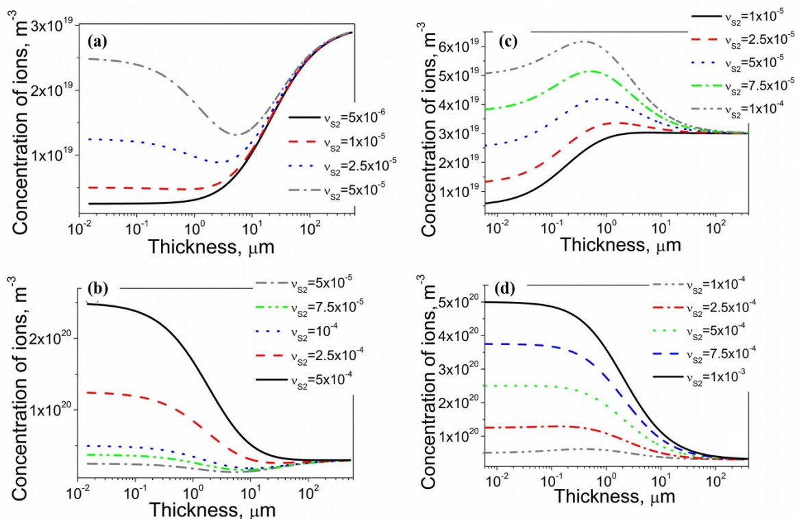
Figure 1. The total concentration of mobile ions, n , as a function of the cell gap calculated at several values of the contamination factor v_{s2} . (a) Monotonous increase (solid and dashed curves) followed by a non-monotonous dependence with a minimum (dotted and dashed-dotted curves). (b) Monotonous decrease (solid and dashed curves) followed by a non-monotonous dependence with a minimum (dotted and dashed-dotted curves). (c) Monotonous increase (solid curve) followed by a non-monotonous dependence with a maximum (other curves). (d) Monotonous decrease (all curves except double-dotted-dashed curve). Additional information can be found in paper [26].
