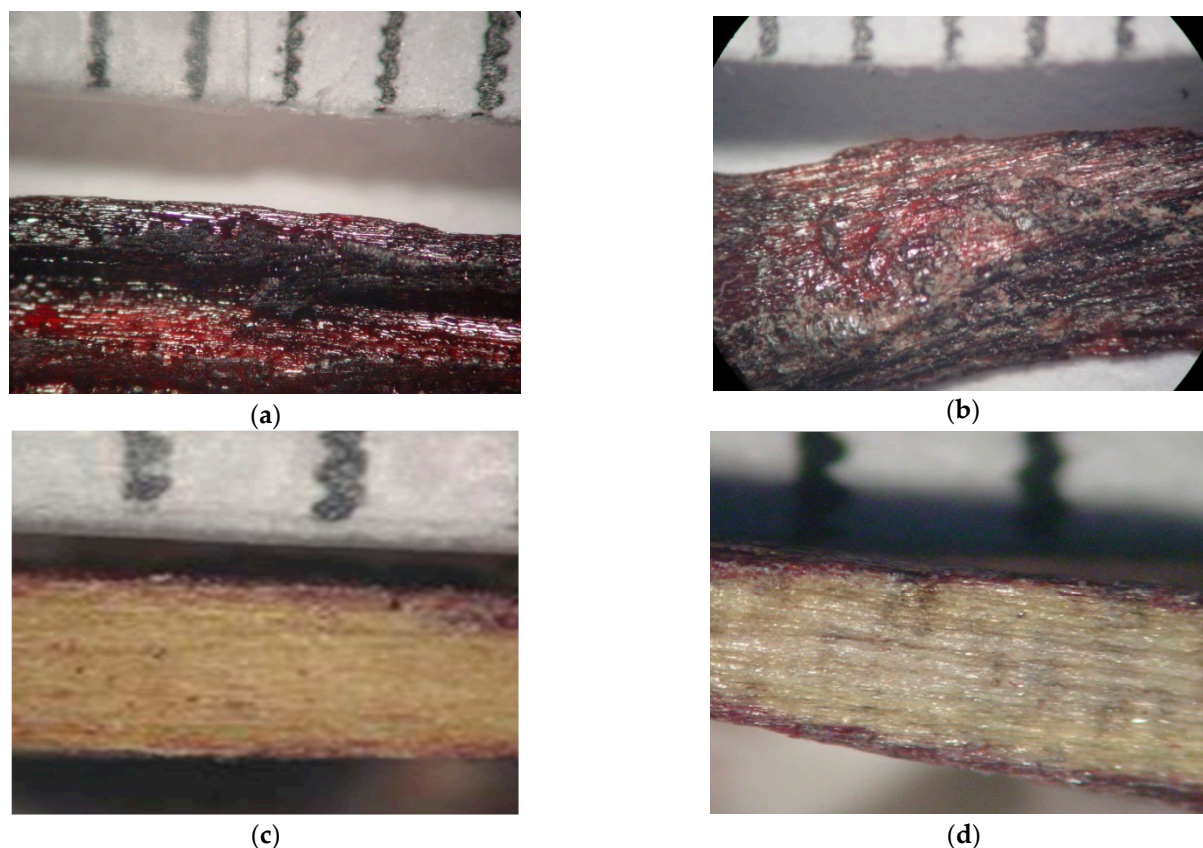
Figure 4. Optical microscope images of (a,c) control PF, and (b,d) PFP20 resin.
