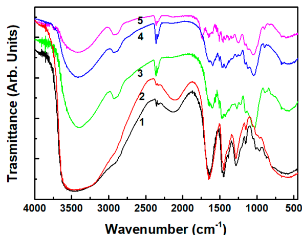
Figure 1. IR spectra of 1: PF, 2: PFP20, 3: PF/woodchips, 4: PFP20/woodchips, and 5: woodchips.
