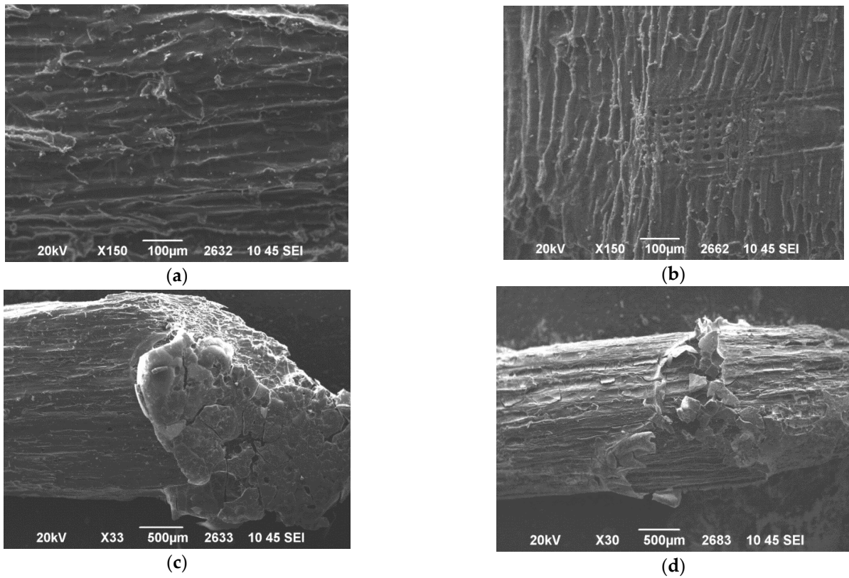
Figure 5. SEM images of (a,c) typical PF, and (b,d) PFP20 resin.
