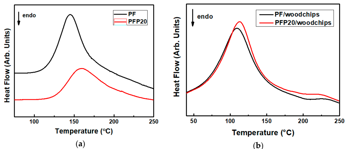
Figure 3. HeatFlow versus temperature of (a) typical PF and PFP20 resin and (b) PF/woodchips and PFP20/woodchips.
