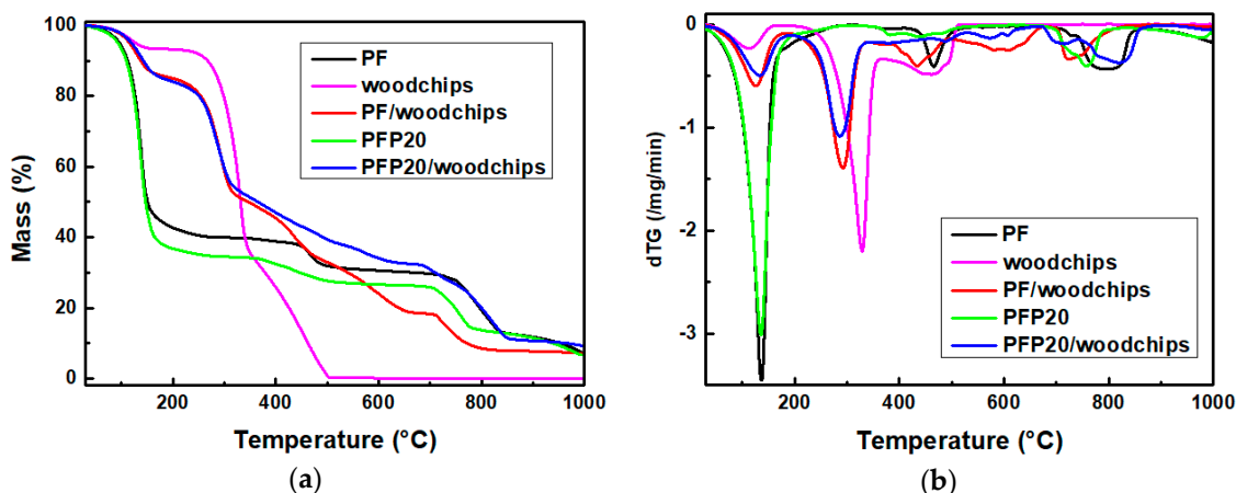
Figure 2. (a) Mass (%) and (b) DTG versus temperature of the typical PF, woodchips, PF/woodchips, PFP20 resin, and PFP20/woodchips.
