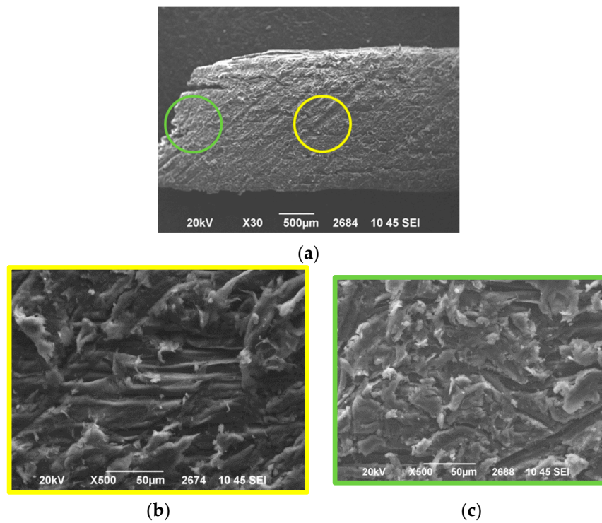
Figure 6. Cross-section SEM images of (a) PFP20/woodchips in (b) the middle (yellow) and (c) at the edge (green) of the sample.
