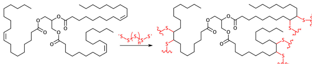
Figure 5. Schematic representation of a polymerization reaction between a triglyceride made up of oleic acid and elemental sulfur [20,21].
