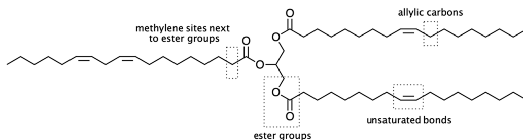
Figure 4. Four main reactive sites of unsaturated triglycerides.
