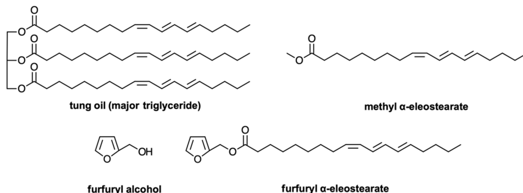
Figure 7. Monomers used for the preparation of tung oil/furfuryl alcohol networks [50].
