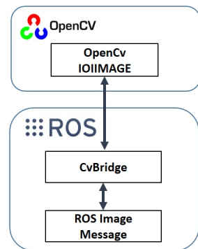
Figure 2. CvBridge/OpenCV communication overall flowchart.
