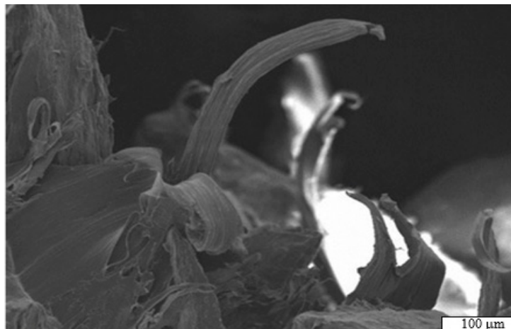
Figure 7. SEM image of the PCL fibers at the fracture face of a tensile test of a 55 wt % DBM/PCL mold sample (the view direction is perpendicular to the XY-plane). Scale bar represents 100 μm.
