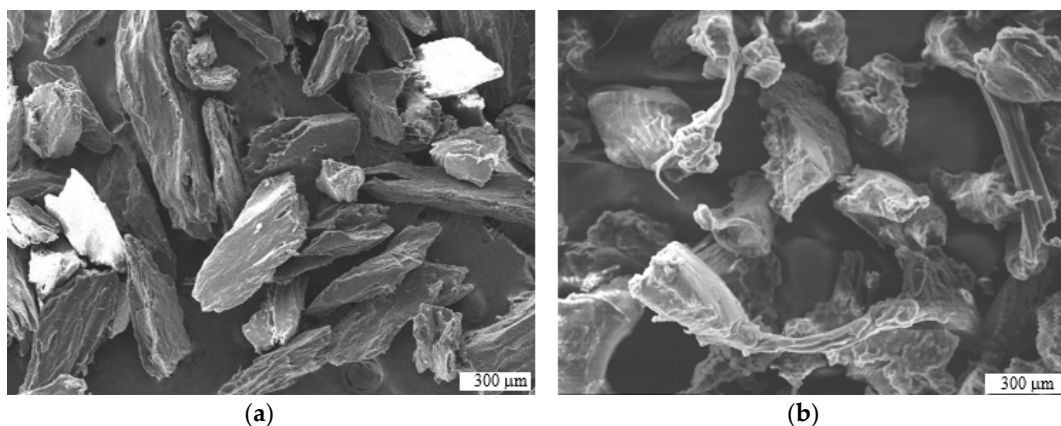
Figure 5. The SEM image of the powders sieved down to <300 µm. (a) Demineralized bone particulates and (b) polycaprolactone (PCL) powders. Scale bars represent 300 µm.
