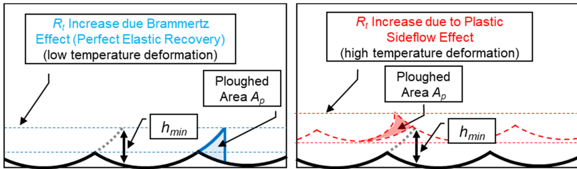
Figure 2. Schematic illustration of the difference between elastic material response (left/blue) and plastic sideflow (right/red), the latter of which is proposed to represent typical thermoplastic material response during machining.
