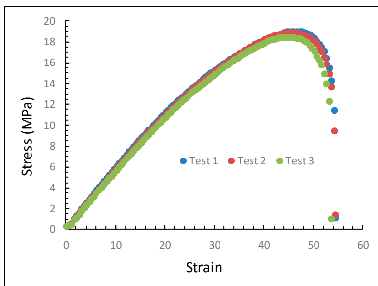
Figure S1. Example of Stress-Strain curves of an original BRC.
