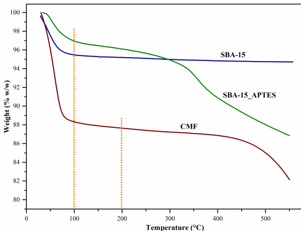
Figure S1. Thermogravimetric analysis of CMF, SBA-15, and SBA-15_APTES.
