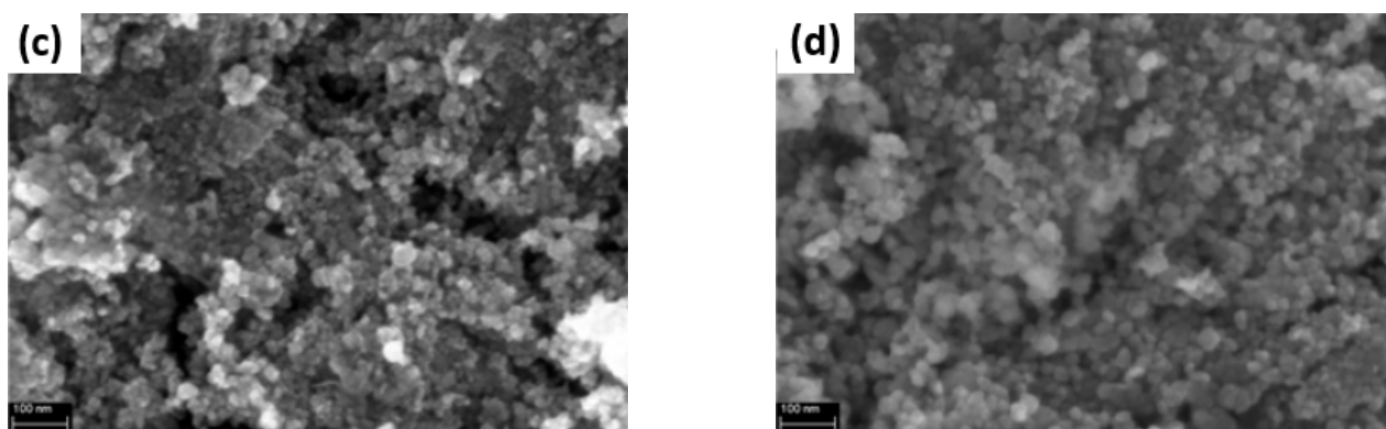
Figure 4. FESEM images of (a) GO (b) MRGO-5, (c) MRGO-10 and (d) MRGO-20.
