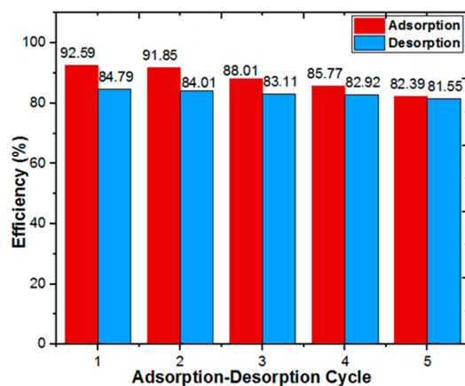
Figure 4. Adsorption–desorption cycle of MO_{C-ZnCl_2} with alkaline solution NaOH (0.01 N).
