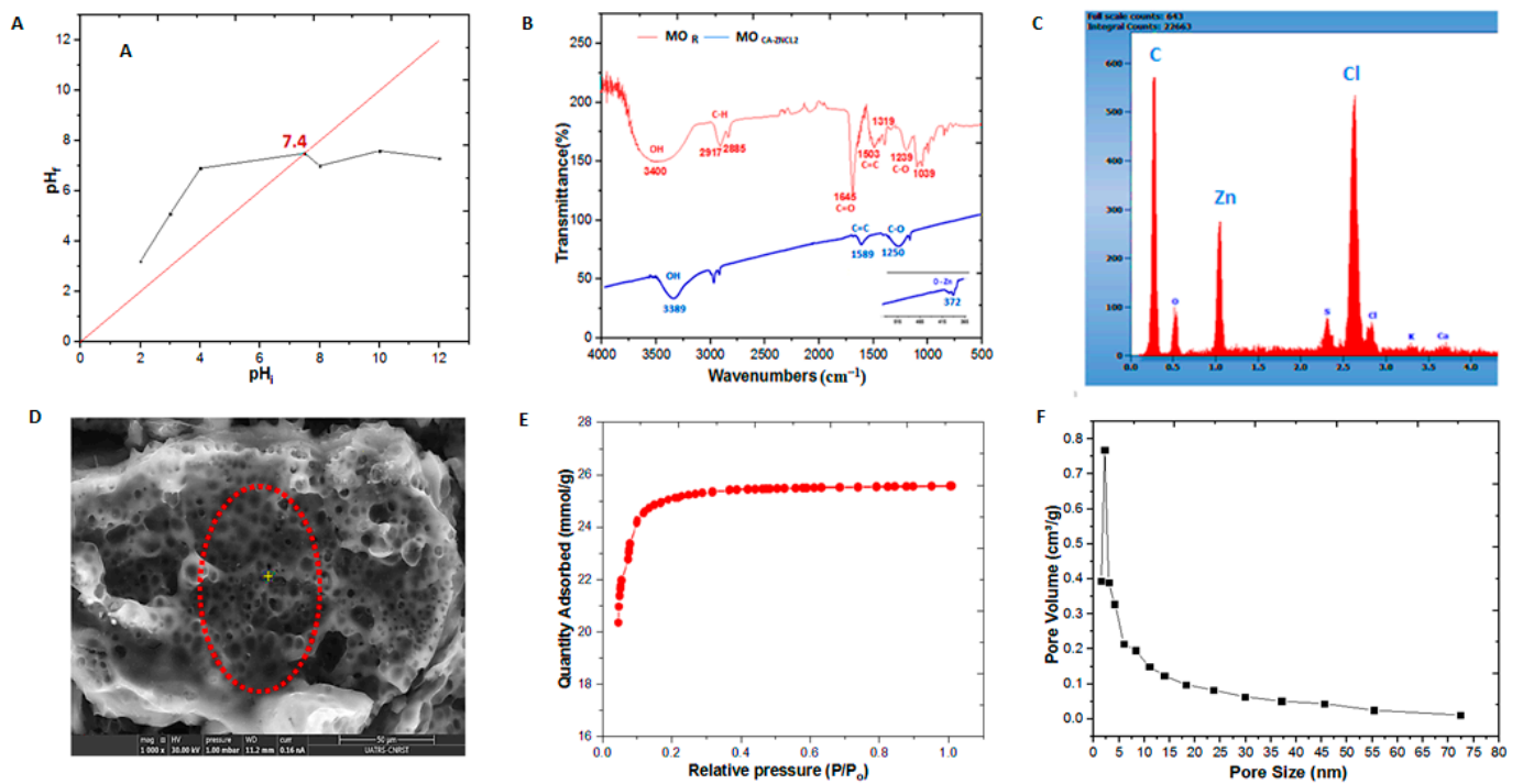
Figure 1. MO C -ZnCl 2 characterization: (A) pH Hpzc , (B) FTIR, (C) EDS, (D) SEM, (E) Adsorption/desorption isotherms of N 2 /77 K, (F) Pore distribution by BJH method.
