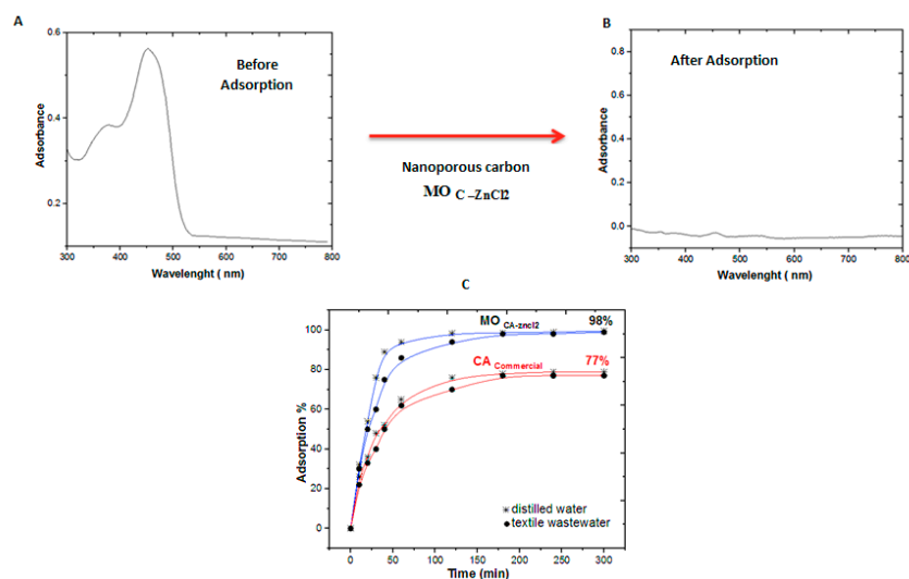
Figure 5. UV-vis spectrophotometer spectra of the dyeing effluent. (A) Before adsorption (B) After adsorption, (C) Comparative adsorption of MO_{C-ZnCl_2} nanoporous carbon vs. commercial activated carbon for MeO adsorption.
