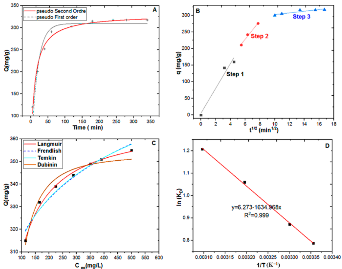
Figure 3. Modeling of adsorption of MeO on \text{MO}_{\text{C-ZnCl}_2} . (A) Kinetics: PFO and PSO, (B) Intraparticle diffusion, (C) Isotherm, (D) Representation of the Van't Hoff line.
