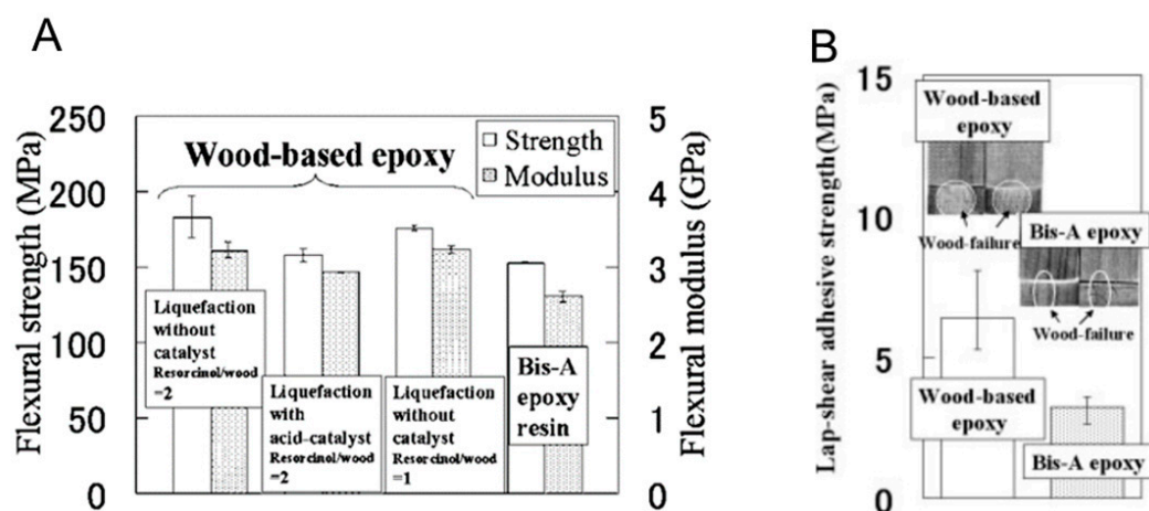
Figure 4. Flexural properties of wood-based epoxy resins (liquefaction time: 1.5 h) (A) and lap-shear adhesive strength of the wood-based epoxy resin (liquefaction time: 1.5 h, resorcino/wood ratio (1:1)) to substrate of plywood (B). In both cases, bisphenol A epoxy resin was used as reference [60].
