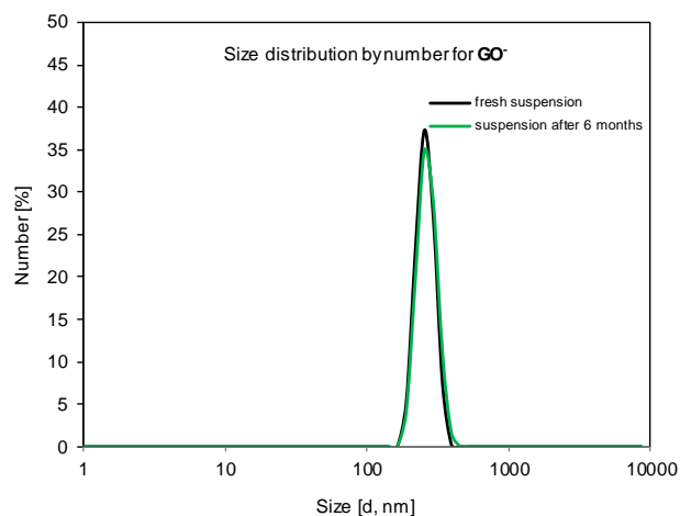
Figure S1. Size distribution measured by DLS for suspensions of \text{GO}^+ - (A) and \text{GO}^- - (B), freshly prepared and after 6 months of storage.
