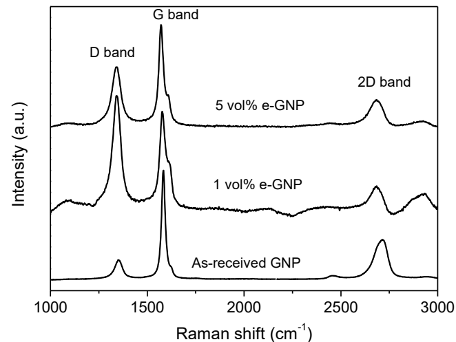
Figure 1. Raman spectra of the yttria tetragonal zirconia (3YTZP) composite powders with 1 and 5 vol.% exfoliated graphene nanoplatelets (e-GNP). The spectrum of the as-received GNP powder is plotted for comparison.
