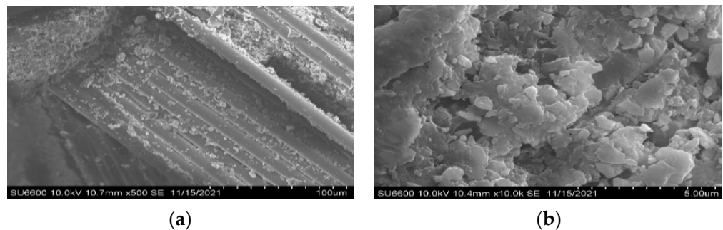
Figure 5. SEM images for 10% SiCE at 10 kV with magnifications (a) 500 (b) 10000.
