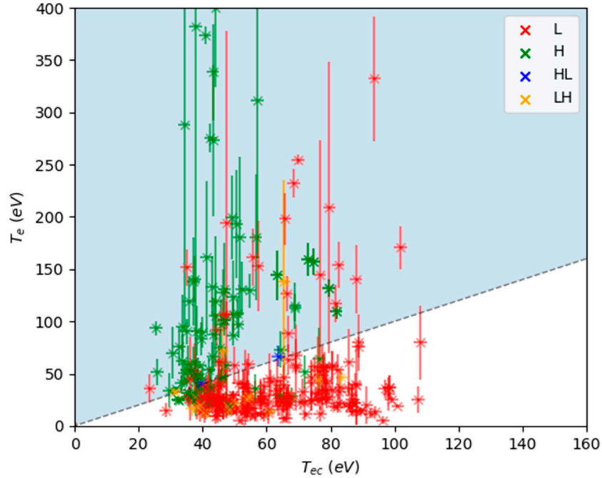
Figure 7. T_e , taken at the point of steepest edge plasma n_e gradient for L-mode, H-mode, L–H transitions and H–L transitions for shots included in the n_e and X-point height scans, plotted as a function of T_{ec} from the finite beta drift wave model. The dotted line represents T_e = T_{ec} .
