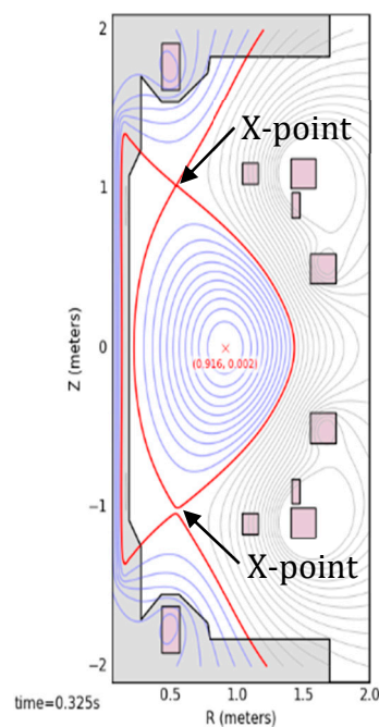
Figure 1. MAST's connected double null magnetic configuration.
