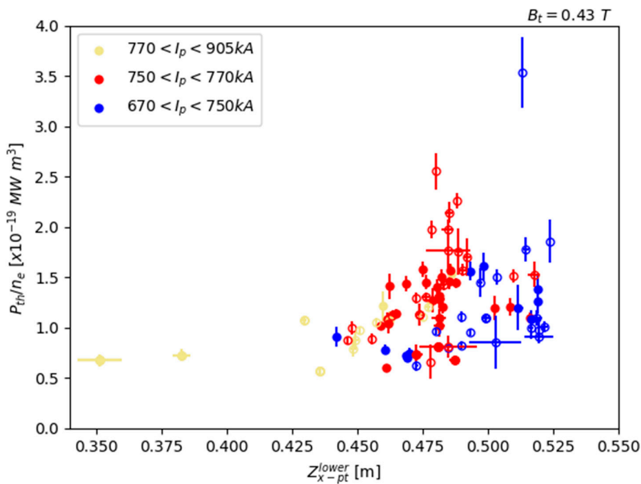
Figure 5. Normalized power threshold for the L–H (closed symbols) and H–L (open symbols), as a function of distance of the lower X-point from the divertor floor for three different values of I_p .
