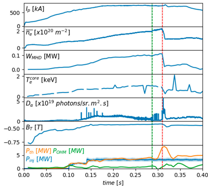
Figure 2. General plasma parameters for a shot 27035 from the density/X-point height scan at 0.7 MA/0.43 T.
