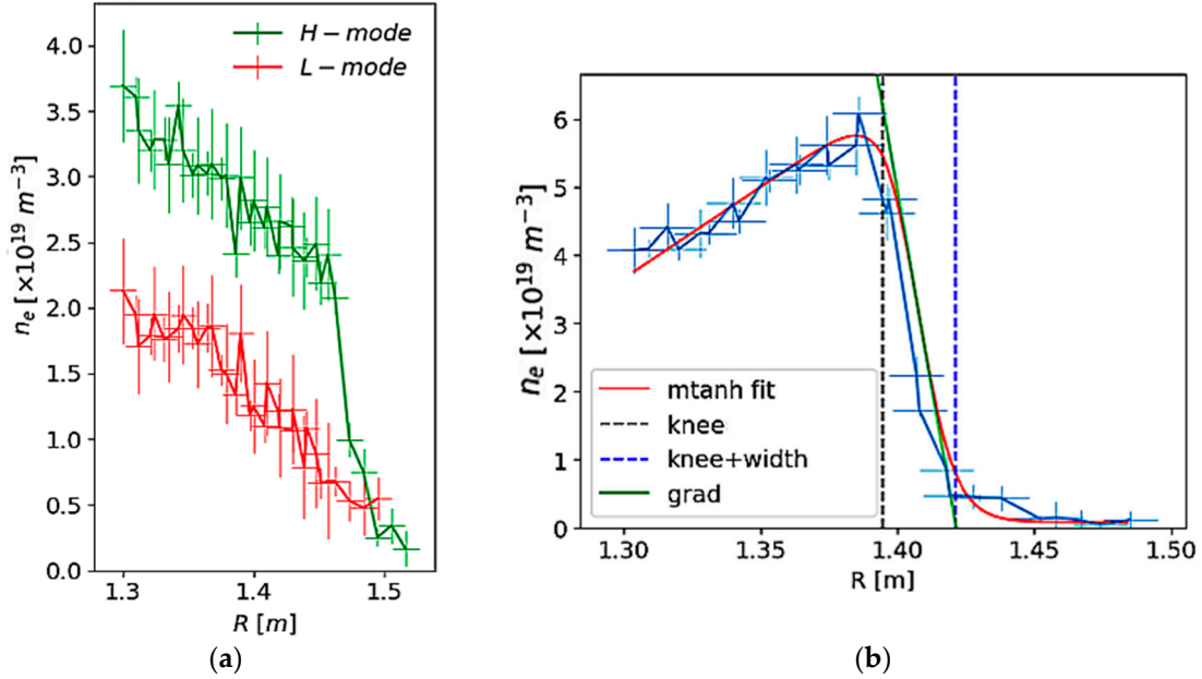
Figure 3. TS measurements on the pedestal n_e for (a) typical L-mode and H-mode profiles for shot number 27035 and (b) with the modified tanh fit to the with the relevant pedestal parameters labeled, knee, width, and steepest n_e gradient.
