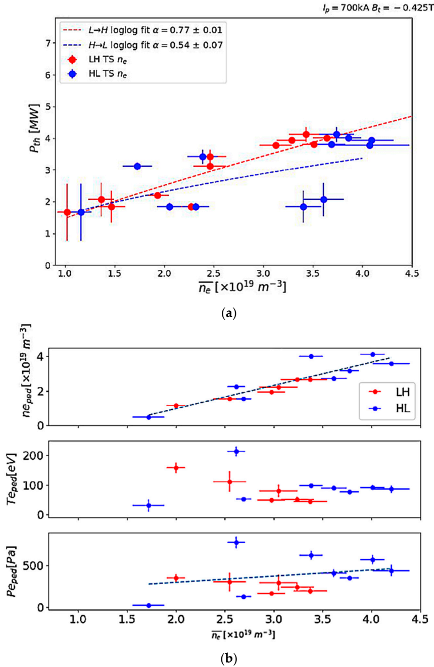
Figure 4. (a) P_{th} for the L–H and H–L transitions and (b) n_e , T_e , and P_e at the n_e pedestal top or knee, plotted as a function of core \bar{n}_e .
