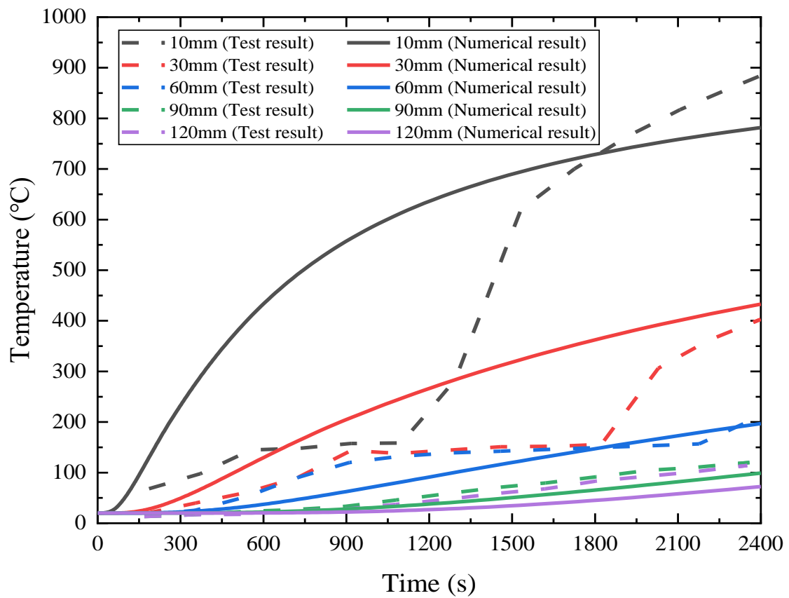
Figure 6. Comparison of the temperature field of specimen RCJ3.
