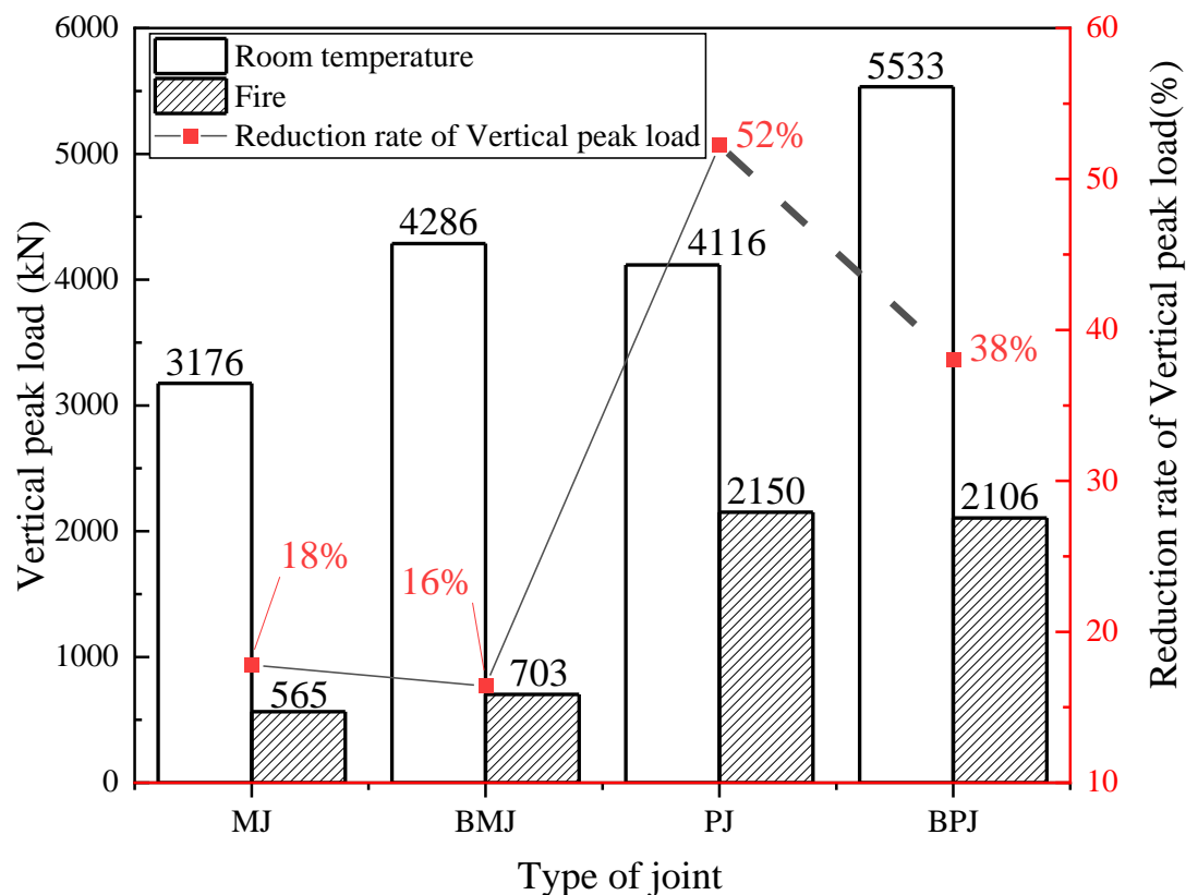
Figure 13. Flexural bearing capacity of four joints under a fire of 120 min and at room temperature.
