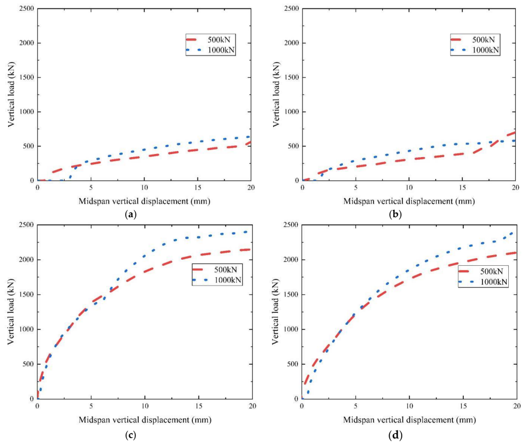
Figure 15. Load–displacement curves of the four joints with different initial axial forces. (a) MJ. (b) BMJ. (c) PJ. (d) BPJ.
