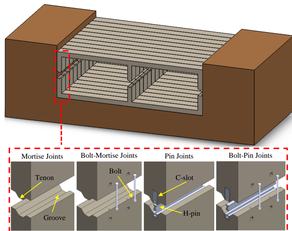
Figure 1. Fabricated frame tunnel joints.
