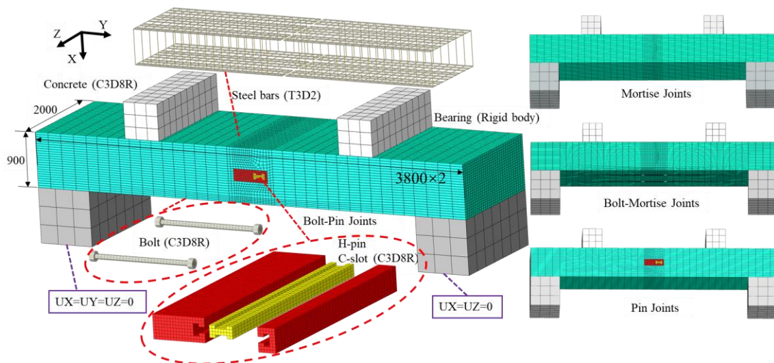
Figure 3. Model mesh (dimensions in mm).
