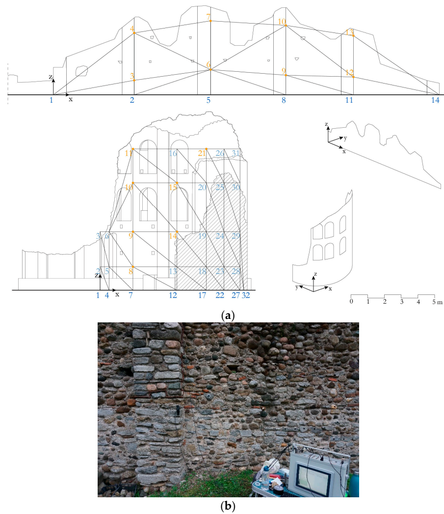
Figure 10. Setup of dynamic identification tests: (a) elevation of the grid for sensor positioning on the north wall and the apse; (b) view of accelerometers and acquisition system.
