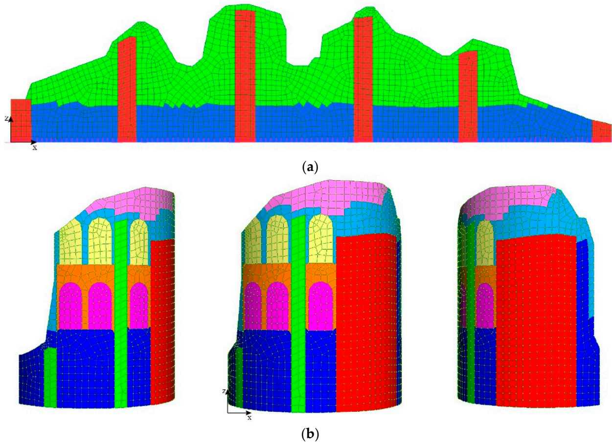
Figure 13. FE models of (a) north wall and (b) main apse. Key to colors in Tables 9 and 10, respectively.
