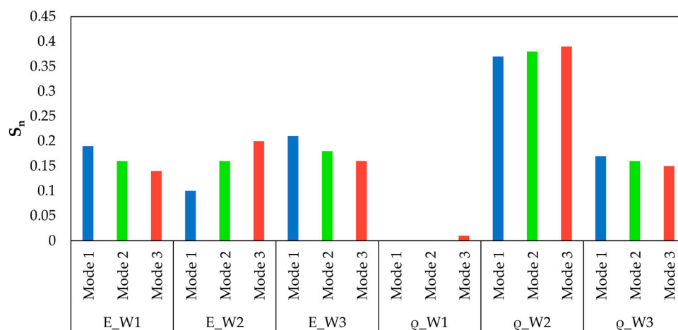
Figure 14. Sensitivity indices ( S_n ) from the variation of elastic modulus E and density \rho in the north wall.
