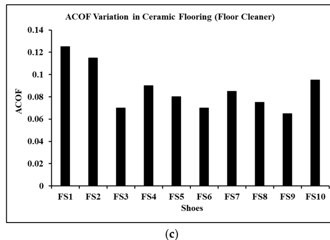
Figure 6. Traction performance of shoes on ceramic flooring in: (a) dry condition, (b) water-contaminated condition, and (c) floor-cleaner-contaminated condition.
