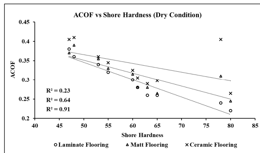
Figure 10. Correlation between shore hardness and ACOF across the shoes in dry slipping condition.
