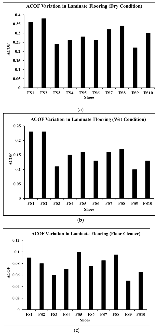
Figure 4. Traction performance of shoes on laminate flooring in: (a) dry condition, (b) water-contaminated condition, and (c) floor-cleaner-contaminated condition.
