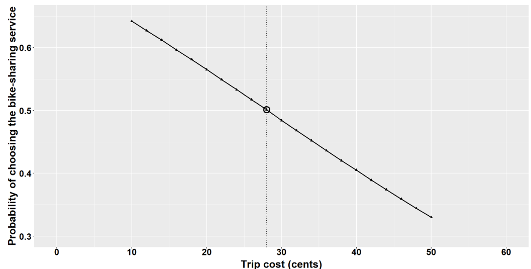
Figure 2. Change in the probability to shift towards the bike-sharing service according to the cost of the service for a trip of 15 min costing 50 cents to use a private car.
