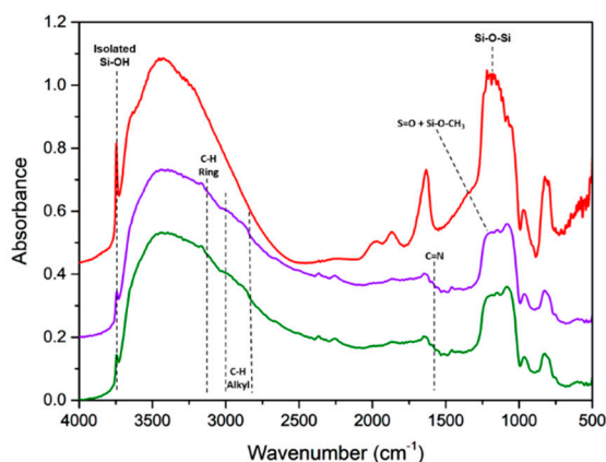
Figure 7. Displaced FTIR spectra of SBA-15 (red), IL-HSO 4 -SBA-15 (green), and IL-Cl-SBA-15 (purple).
