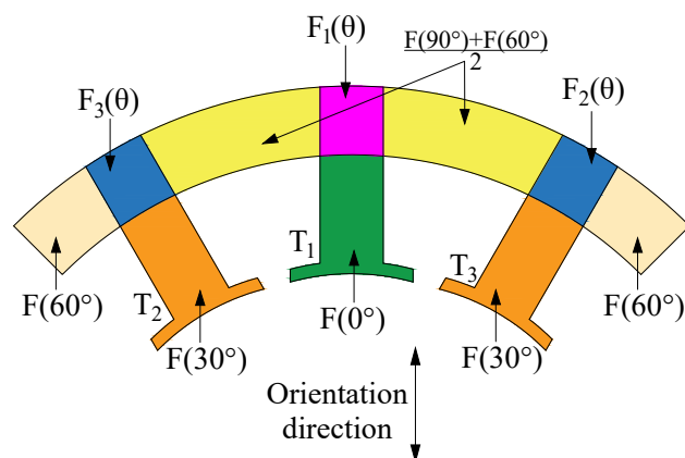
Figure 38. Equivalent piecewise isotropic model for one segment, with each color representing a different angle away from the rolling direction. The model consists of three isotropic segments: (1) stator tooth, (2) back iron behind stator slot, and (3) back iron behind stator tooth. Figure adapted from [155].
