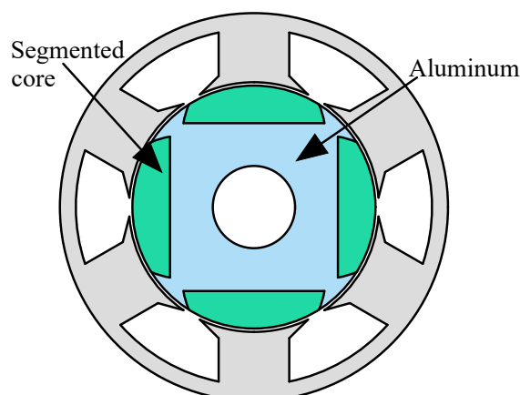
Figure 16. Construction of segmented rotor SRM with solid aluminum block in rotor. Figure adapted from [91].
