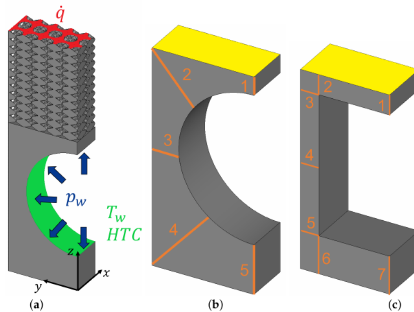
Figure 3. (a) Representation of the geometric domain of the 3D model and the applied boundary conditions. In order to save a considerable amount of computational resources, only half of the PFU was reproduced in the solid model, using the symmetry of the geometry with respect to the x - z plane; (b,c) paths traced within the heat sink geometry for the structural verifications required by SDC-IC standards, for Configurations 1 and 2, respectively.
