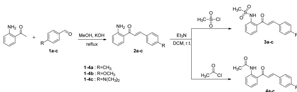
Scheme 2. Synthesis of the 2'-aminochalcones 2a–c , 3a–c and 4a–c .
