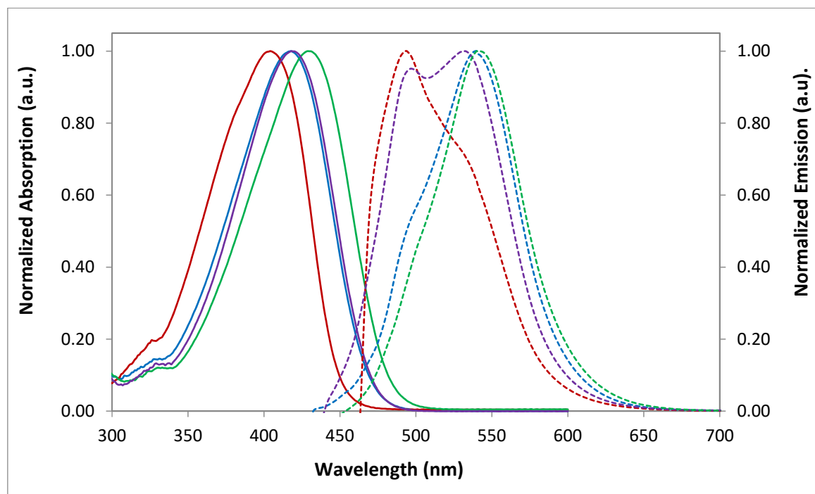
Figure 3. Normalized absorption and emission spectra of chalcone 2c in acetonitrile, diethyl ether, chloroform and dimethyl sulfoxide ( \lambda_{exc} = 418 nm, 404 nm, 418 nm and 429 nm, respectively; absorption, full line; emission, dotted line).
