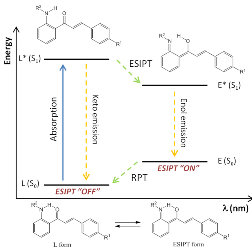
Scheme 1. Description of the Excited State Intramolecular Proton Transfer (ESIPT) process [16].
