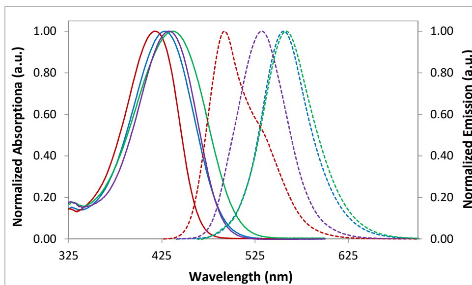
Figure 4. Normalized absorption and emission spectra of chalcone 4c in acetonitrile, diethyl ether, chloroform and dimethyl sulfoxide ( \lambda_{exc} = 428 nm, 417 nm, 432 nm and 437 nm, respectively; absorption, full line; emission, dotted line).
