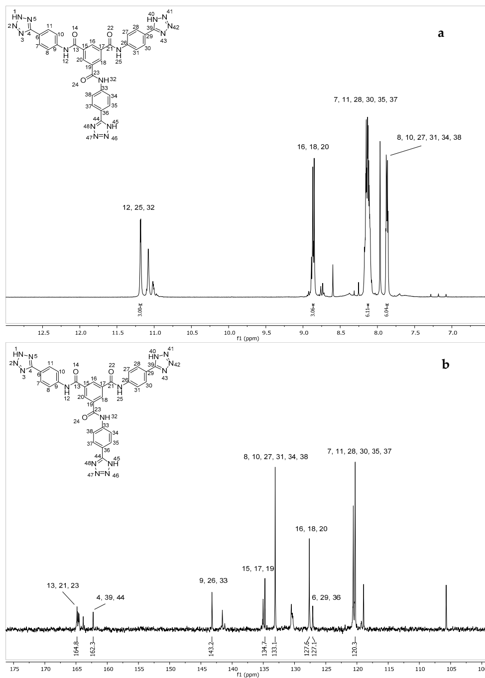
Figure 4. (a) ^1\text{H} NMR spectrum and (b) ^{13}\text{C} NMR spectrum of ligand 7.
