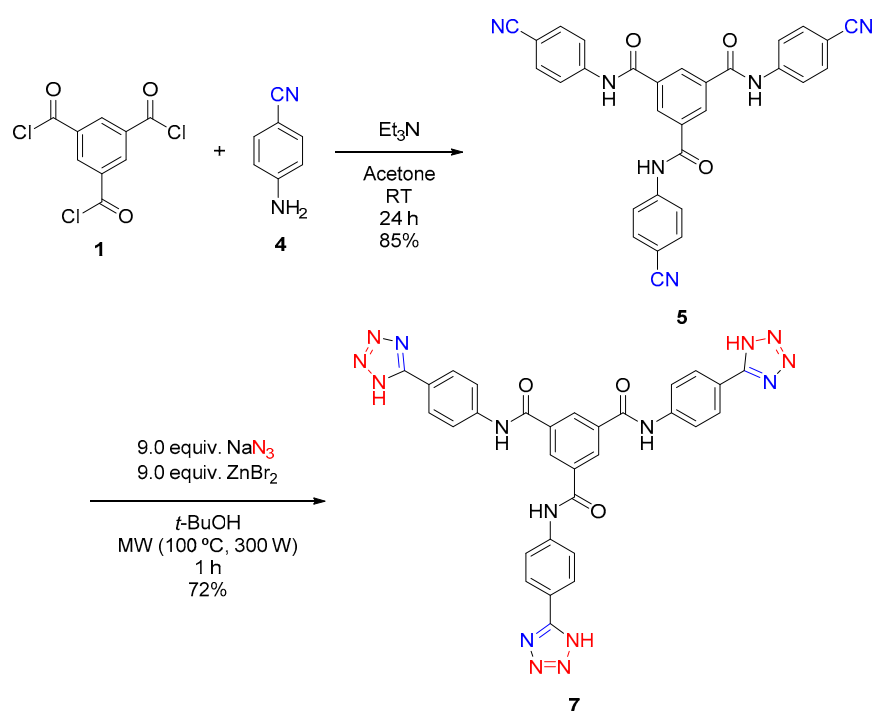
Scheme 2. Synthesis of ligands 5 and 7 .
