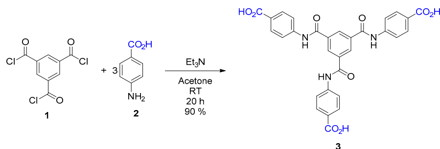
Scheme 1. Synthesis of ligand 3 .
