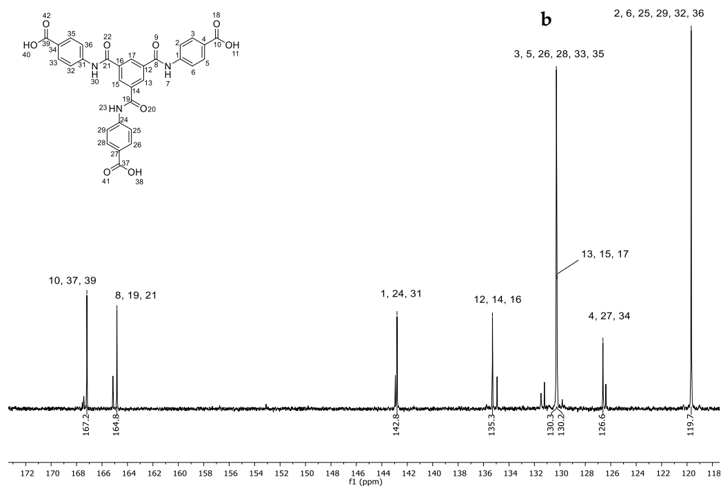
Figure 2. (a) ^1\text{H} NMR spectrum and (b) ^{13}\text{C} NMR spectrum of ligand 3.
