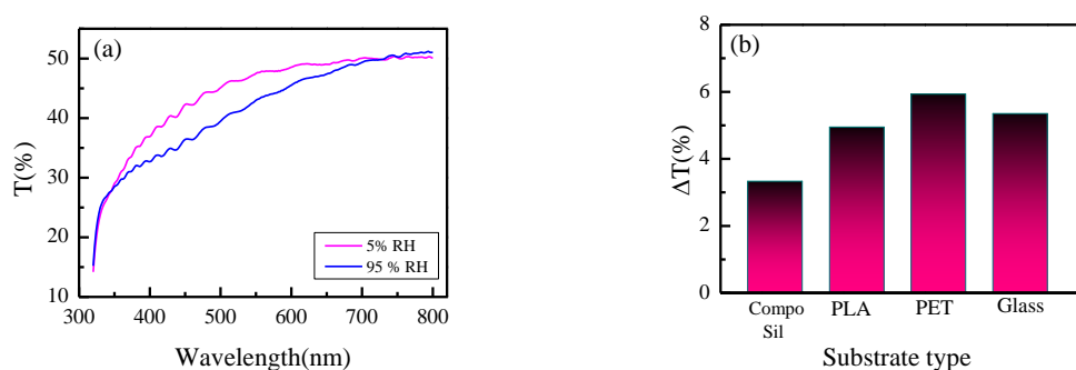
Figure 3. (a) Measured transmission spectra of PET substrate with deposited Au:Pd/PVA-Ac24 when exposed to low (magenta) and high (blue) relative humidity; (b) Transmittance change, \Delta T_{max} (%) calculated from measured transmission spectra of Compo-Sil, PLA, PET and glass substrates with deposited Au:Pd/PVA-Ac24 at low and high relative humidity.
