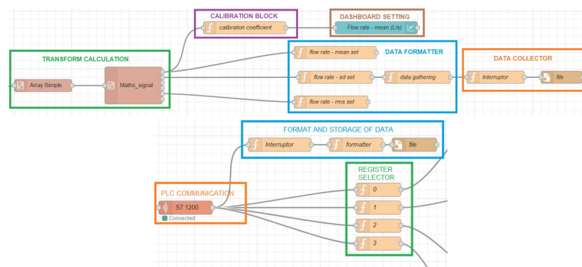
Figure 2. Node-RED data integration.
