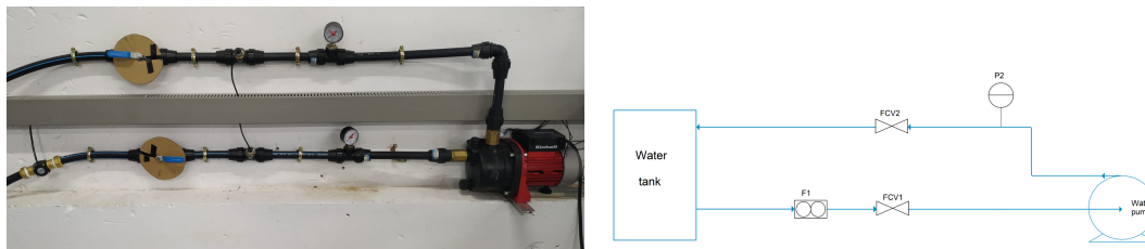
Figure 1. Image and schematic representation of the test bench.
