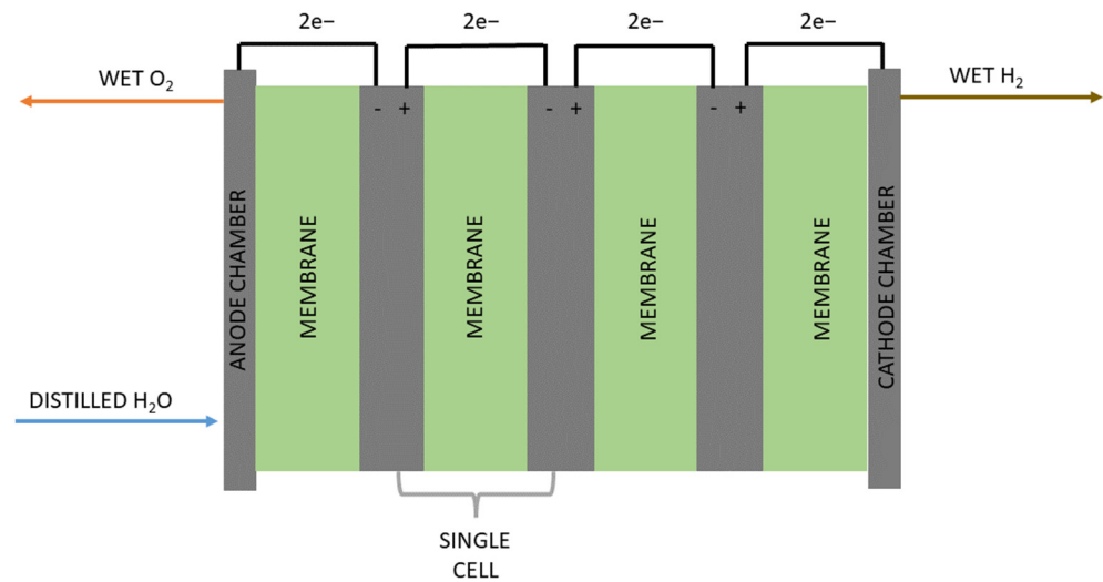
Figure 1. Structure and operation of a PEMEL.
