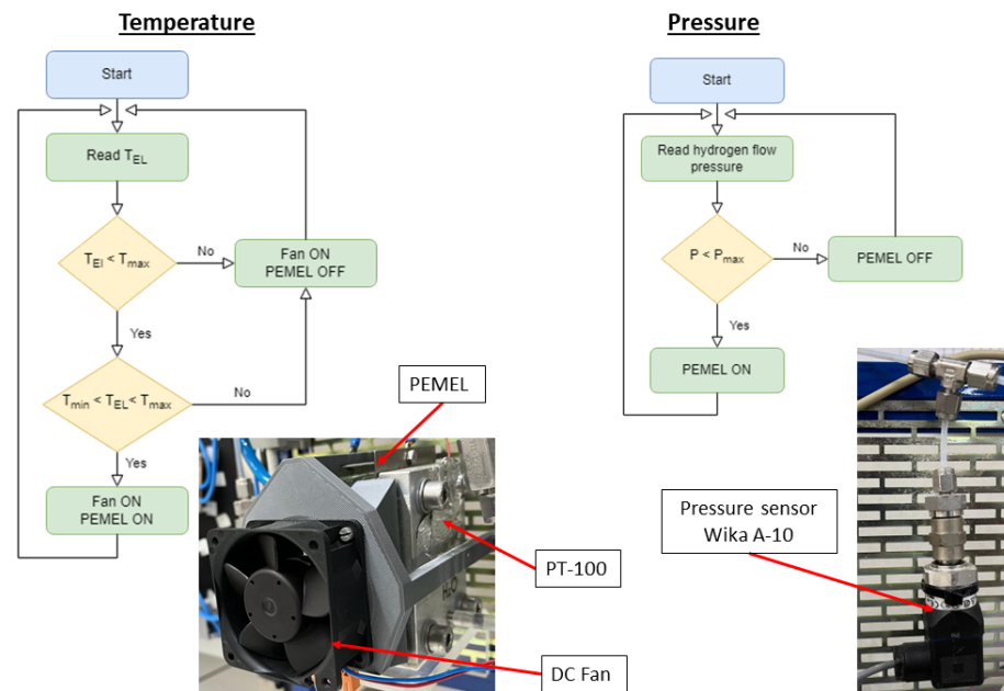
Figure 3. Control algorithms for temperature and pressure and equipment involved.
