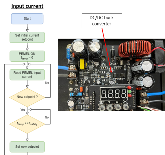
Figure 5. Control algorithms for the PEMEL input current and the related DC/DC converter.
