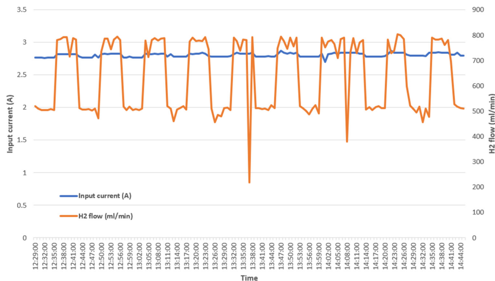
Figure 6. Input current and H 2 flow curve.
