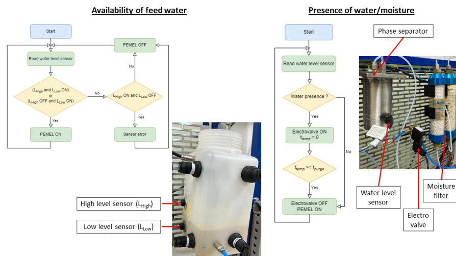
Figure 4. Control algorithms for feed water and presence of moisture. Equipment involved.
