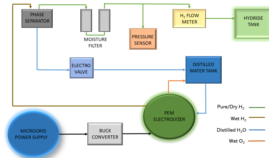
Figure 2. PEMEL hydrogen generation system.
