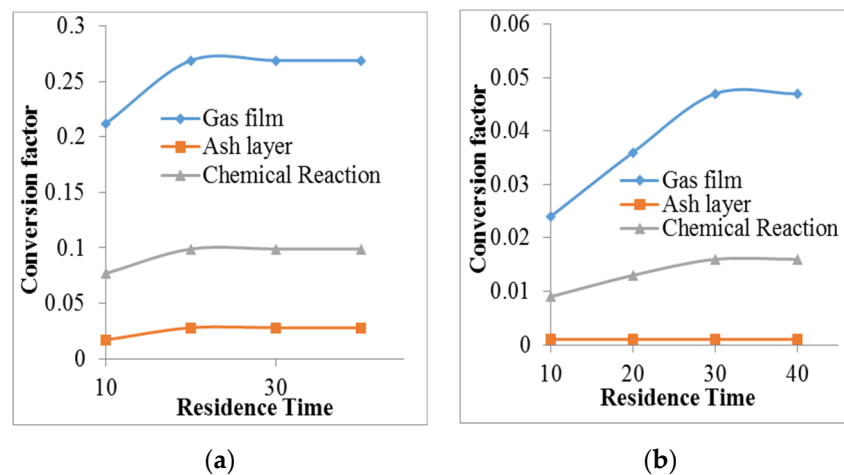
Figure 6. Determination of rate control stages based on the conversion factor for iron-ore samples of different size ranges at 900 °C. (a) 10–14.99 mm; (b) 15–20 mm.
