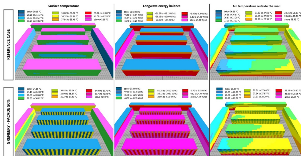
Figure 2. Distribution of surface temperature [°C], longwave energy balance [W/m 2 ] and air temperature outside the wall [°C] (southern) for both reference and vertical greening at 50% cases.
