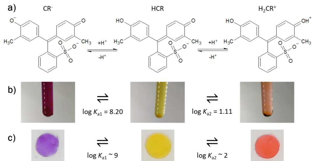
Figure 1. Protonation equilibria of o-cresol red (a), color evolution in solution ( \sim 10 \mu\text{M} ) and correspondent \log K_a , as found in the literature [33,34] (b) and CR-EVOH@ sensors coloration and apparent \log K_a after functionalization, estimated from background experiments [29,31,32] (c).
